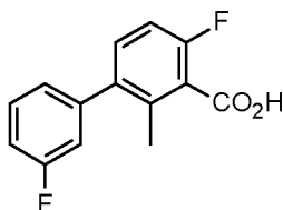
6-Fluoro-3-(3-fluorophenyl)-2-methylbenzoic acid (III(o))
