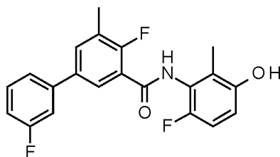
2-Fluoro-N-(6-fluoro-3-hydroxy-2-methyl-phenyl)-5-(3-fluorophenyl)-3-methyl-benzamide
