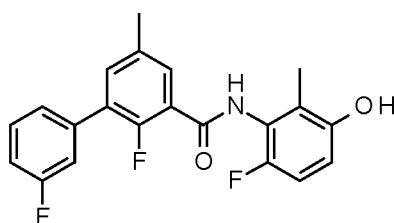
2-Fluoro-N-(6-fluoro-3-hydroxy-2-methyl-phenyl)-3-(3-fluorophenyl)-5-methyl-benzamide
