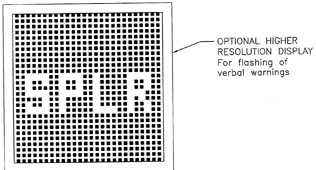
DETAILED VIEW FRONT OF DISPLAY
