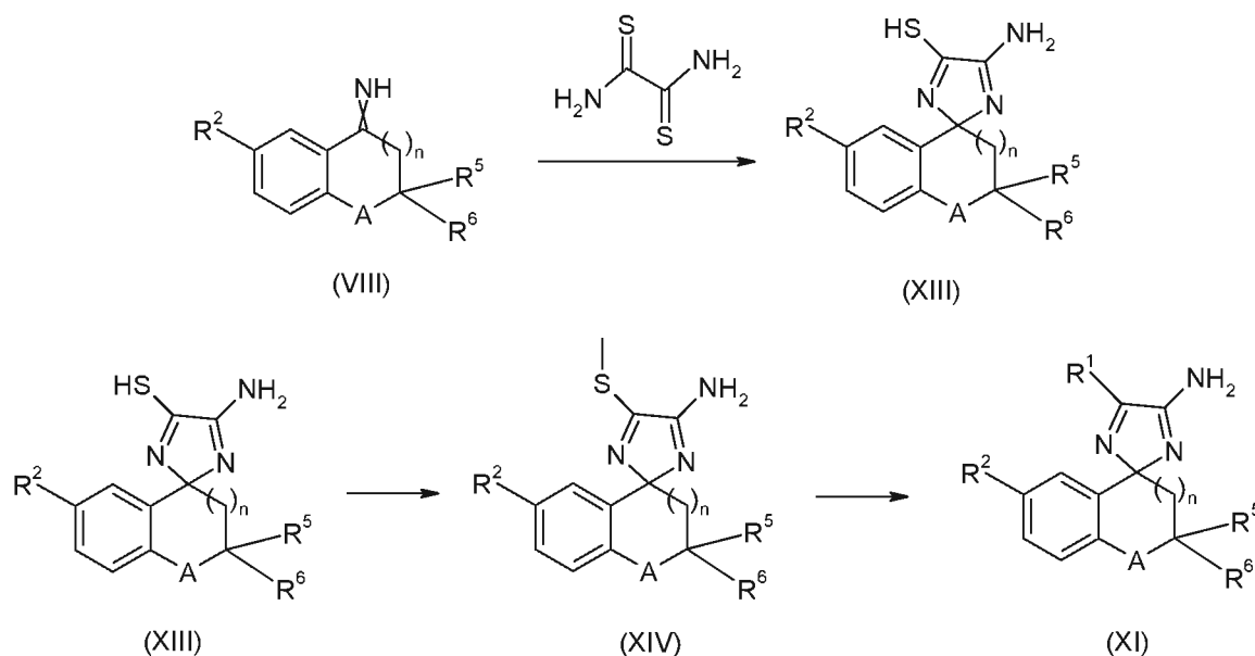
Scheme 6
