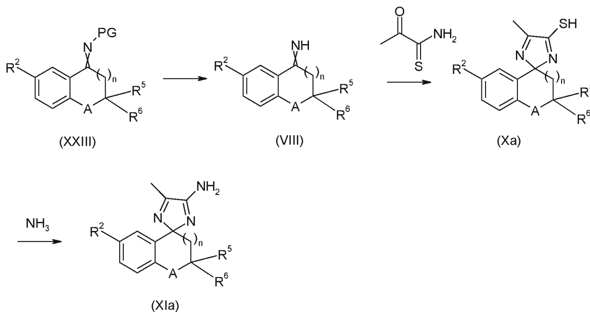
Scheme 10
