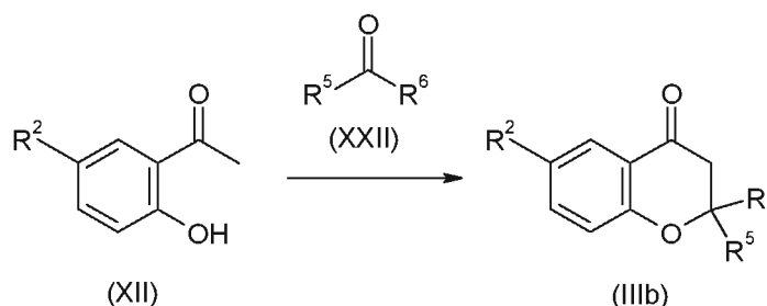
Scheme 16
