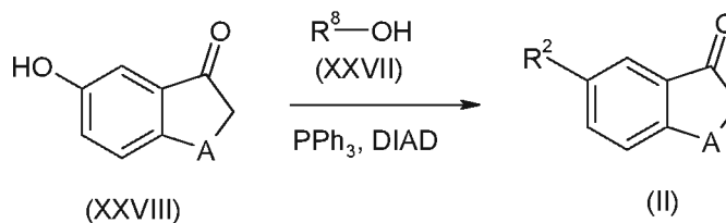
Scheme 19
