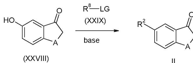
Scheme 18
