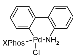
precatalyst 13
