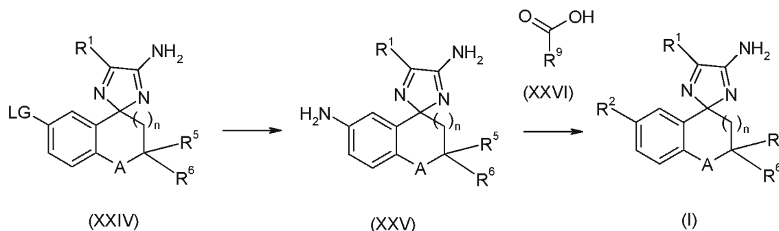
Scheme 15
