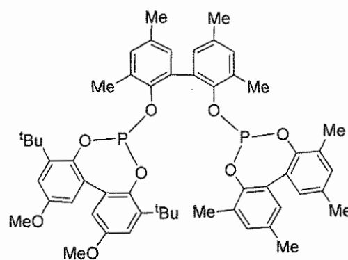
ligand (1Ia)
