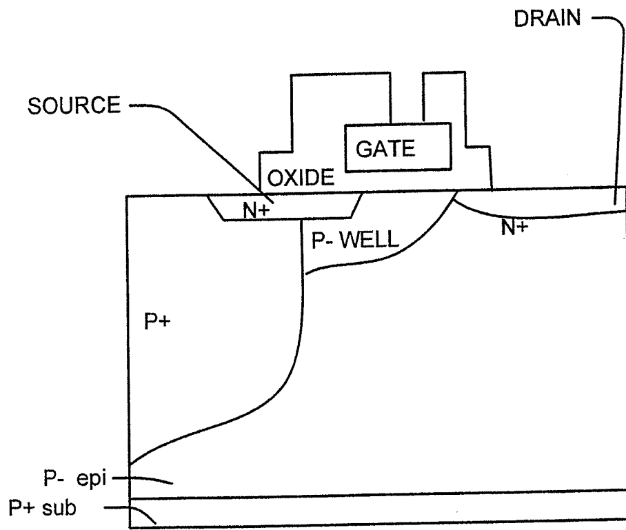
NON-OFFSET LDMOS
