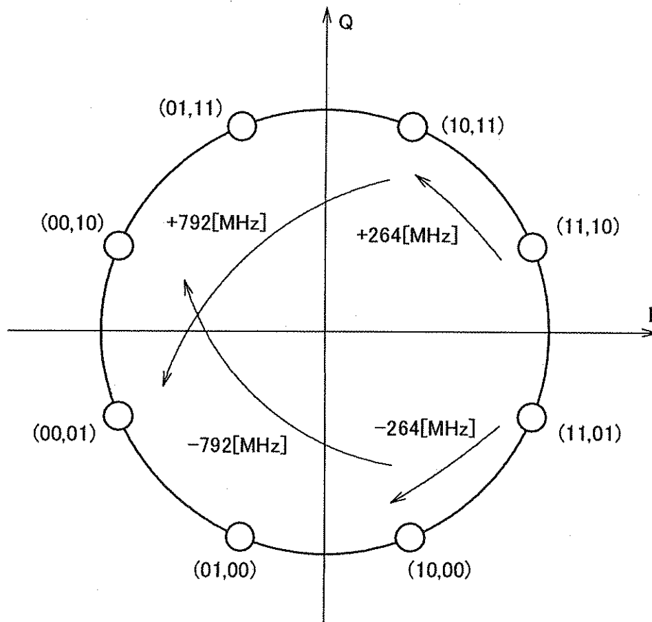
COMPLEX AMPLITUDE VALUES OF DA CONVERTERS
