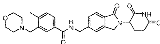
N-((2-(2,6-dioxopiperidin-3-yl)-1-oxoisoindolin-5-yl)methyl)-4-methyl-3-(morpholinomethyl)benzamide;
