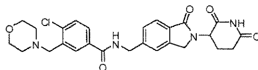
4-chloro-N-((2-(2,6-dioxopiperidin-3-yl)-1-oxoisoindolin-5-yl)methyl)-3-(morpholinomethyl)benzamide;
