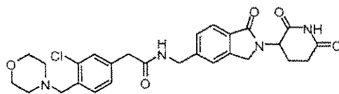
2-(3-chloro-4-(morpholinomethyl)phenyl)-N-((2-(2,6-dioxopiperidin-3-yl)-1-oxoisindolin-5-yl)methyl)acetamide;
