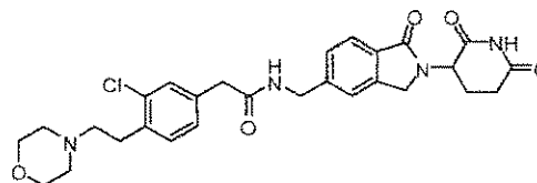
2-(3-chloro-4-(2-morpholinoethyl)phenyl)-N-((2-(2,6-dioxopiperidin-3-yl)-1-oxoisindolin-5-yl)methyl)acetamide;
