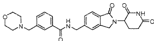
N-((2-(2,6-dioxopiperidin-3-yl)-1-oxoisoindolin-5-yl)methyl)-3-(morpholinomethyl)benzamide;
