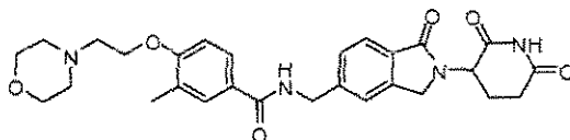
N-((2-(2,6-dioxopiperidin-3-yl)-1-oxoisindolin-5-yl)methyl)-3-methyl-4-(2-morpholinoethoxy)benzamide;
