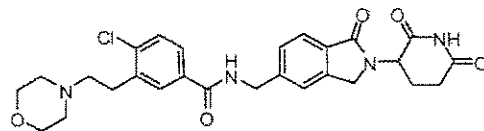
4-chloro-N-((2-(2,6-dioxopiperidin-3-yl)-1-oxoisoindolin-5-yl)methyl)-3-(2-morpholinoethyl)benzamide;
