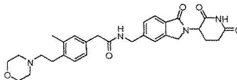
N-((2-(2,6-dioxopiperidin-3-yl)-1-oxoisindolin-5-yl)methyl)-2-(3-methyl-4-(2-morpholinoethyl)phenyl)acetamide;
