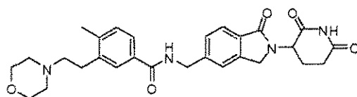
N-((2-(2,6-dioxopiperidin-3-yl)-1-oxoisoindolin-5-yl)methyl)-4-methyl-3-(2-morpholinoethyl)benzamide;
