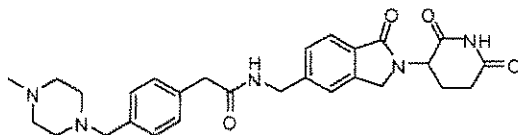
N-((2-(2,6-dioxopiperidin-3-yl)-1-oxoisindolin-5-yl)methyl)-2-(4-((4-methylpiperazin-1-yl)methyl)phenyl)acetamide;
