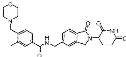
N-((2-(2,6-dioxopiperidin-3-yl)-1-oxoisindolin-5-yl)methyl)-3-methyl-4-(morpholinomethyl)benzamide;
