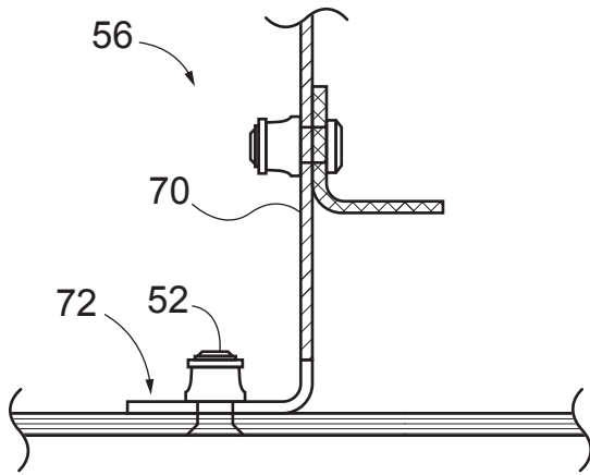
FIG. 6 (PRIOR ART)
