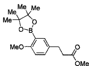
Intermediate H
