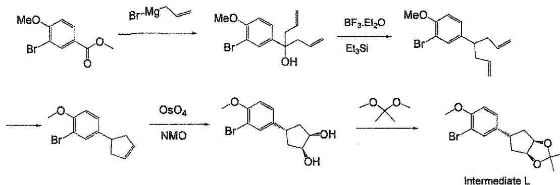
Scheme L
