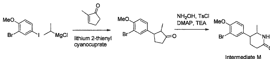
Scheme M
