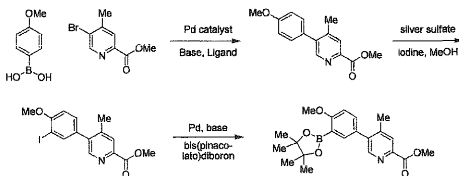
Scheme F
