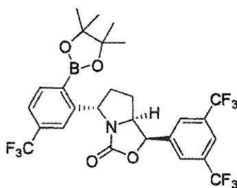
(1R,5S,7aS)-1-(3,5-bis(trifluoromethyl)phenyl)-5-(2-(4,4,5,5-tetramethyl-1,3,2-dioxaborolan-2-yl)-5-(trifluoromethyl)phenyl)tetrahydropyrrolo[1,2-c]oxazol-3(1H)-one
