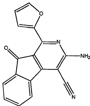
9H-indeno[2,1-c]pyridine-4-carbonitrile, 3-amino-1-furan-2-yl-9-oxo-
