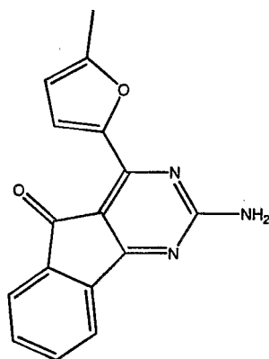
2-amino-4-(5-methyl-furan-2-yl)-indeno[1,2-d]pyrimidin-5-one
