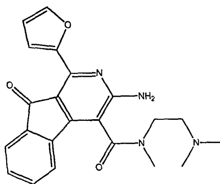
9H-indeno[2,1-c]pyridine-4-carboxylic acid, 3-amino-1-furan-2-yl-9-oxo-, (2-dimethylamino-1-methyl-ethyl)-amide
