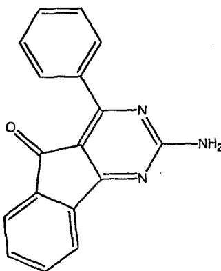
2-amino-4-phenyl-indeno[1,2-d]pyrimidin-5-one
