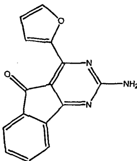
2-amino-4-furan-2-yl-indeno[1,2-d]pyrimidin-5-one
