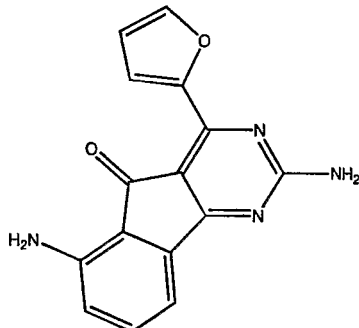
2,6-diamino-4-furan-2-yl-indeno[1,2-d]pyrimidin-5-one
