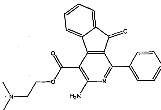
5 9H-indeno[2,1-c]pyridine-4-carboxylic acid, 3-amino-1-phenyl-9-oxo-, 2-dimethylamino-ethyl ester
