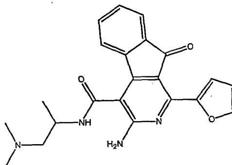
9H-indeno[2,1-c]pyridine-4-carboxylic acid, 3-amino-1-furan-2-yl-9-oxo-, (2-dimethylamino-1-methyl-ethyl)-amide
