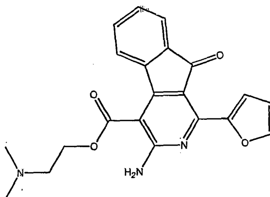
9H-indeno[2,1-c]pyridine-4-carboxylic acid, 3-amino-1-furan-2-yl-9-oxo-, 2-dimethylamino-ethyl ester
