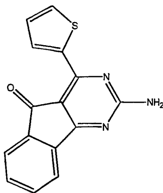
2-amino-4-thiophen-2-yl-indeno[1,2-d]pyrimidin-5-one
