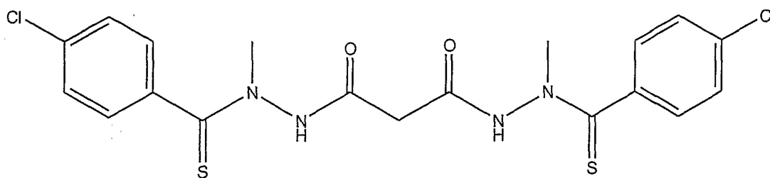
Compound (3)
