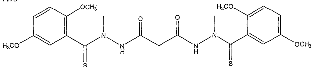
Compound (2)
