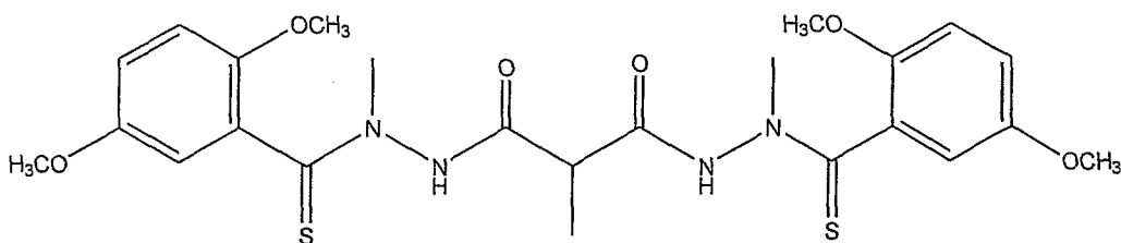
Compound (5)
