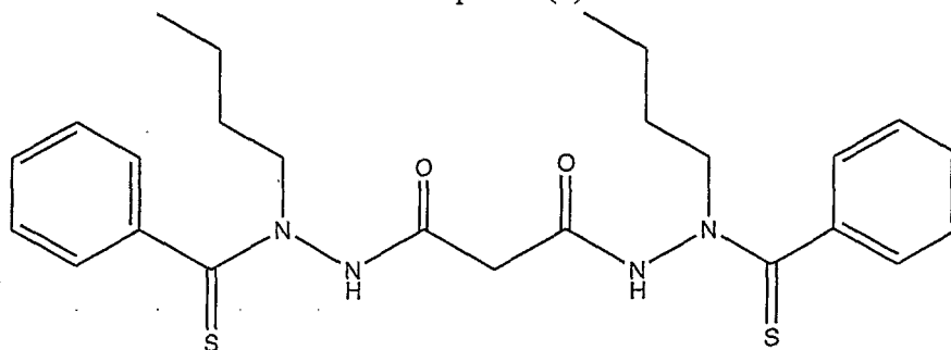
Compound (4)
