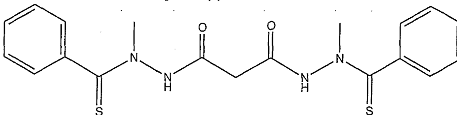
Compound (1)
