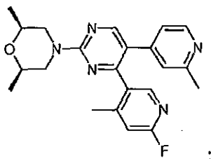
cis -2-[2-(2,6-Dimethyl-4-morpholinyl)-5-(2-methyl-4-pyridinyl)-4-pyrimidinyl]-4-fluorobenzonitrile
