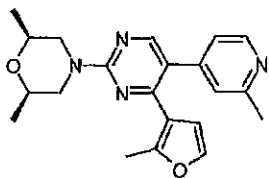
trans -2,6-Dimethyl-4-[4-(2-methyl-3-furanyl)-5-(2-methyl-4-pyridinyl)-2-pyrimidinyl]morpholine
