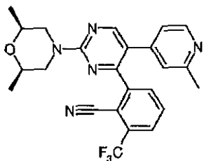
cis -2-[2-(2,6-dimethyl-4-morpholinyl)-5-(2-methyl-4-pyridinyl)-4-pyrimidinyl]-6-(trifluoromethyl)benzonitrile
