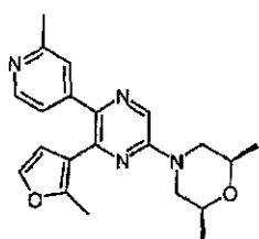
6-( cis -2,6-dimethyl-4-morpholinyl)-2'-methyl-4-(2-methyl-3-furanyl)-3,4'-bipyridine
