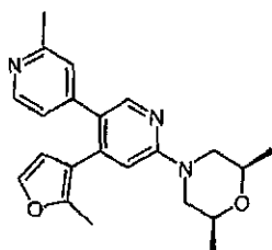
6-( cis -2,6-dimethyl-4-morpholinyl)-2'-methyl-2-(2-methyl-3-furanyl)-3,4'-bipyridine
