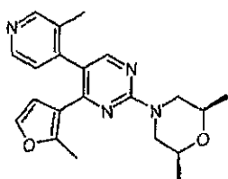
cis -2,6-Dimethyl-4-{5-(2-methyl-4-pyridinyl)-4-[2-(trifluoromethyl)-3-pyridinyl]-2-pyrimidinyl}morpholine
