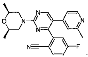
cis -2-[2-(2,6-dimethyl-4-morpholinyl)-5-(2-methyl-4-pyridinyl)-4-pyrimidinyl]-6-(trifluoromethyl)benzonitrile
