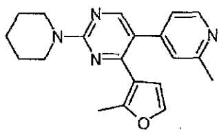
cis -2,6-Dimethyl-4-[4-(2-methyl-3-furanyl)-5-(2-methyl-4-pyridinyl)-2-pyrimidinyl]morpholine
