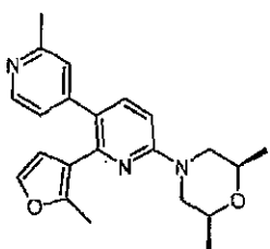
cis -2,6-Dimethyl-4-[3-(2-methyl-3-furanyl)-4-(2-methyl-4-pyridinyl)phenyl]morpholine
