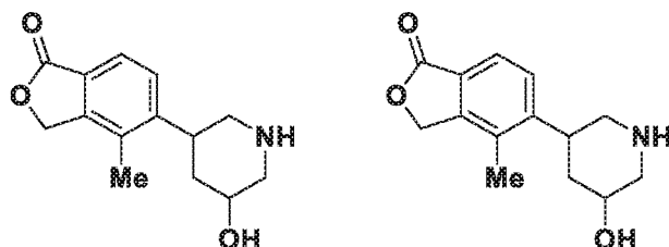
Diastereomer-I (118A) Diastereomer-II (118B)
