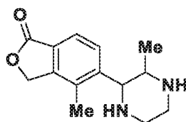
Enantiomer-II (71-II)
