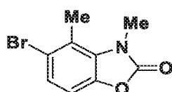
Intermediate 82:
