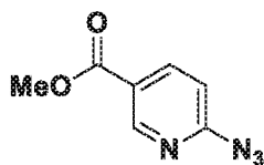
Intermediate 152A: methyl 6-azidonicotinate
