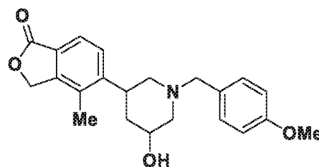
Diastereomer-II (122F)
