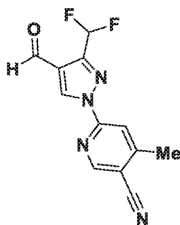
Intermediate 157A: (3-(difluoromethyl)-1H-pyrazol-4-yl)methanol
