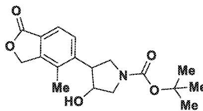
Diastereomer-II (106C)
