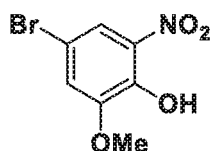
Intermediate 35A: 4-bromo-2-methoxy-6-nitrophenol
