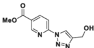
Intermediate 152B: methyl 6-(4-(hydroxymethyl)-1H-1,2,3-triazol-1-yl)nicotinate
