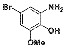
Intermediate 35B: 2-amino-4-bromo-6-methoxyphenol
