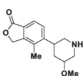
Diastereomer-I (119A)
