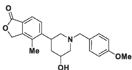
Diastereomer-I (122E)
