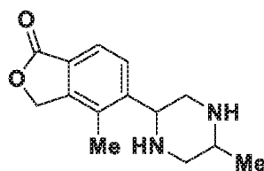
Enantiomer-II (153-II)
