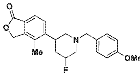
Enantiomer-I (122G-II)
