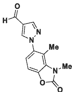
Intermediate 82: 1-(3,4-dimethyl-2-oxo-2,3-dihydrobenzo[d]oxazol-5-yl)-1H-pyrazole-4-carbaldehyde
