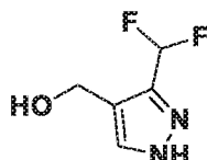
Intermediate 157A: (3-(difluoromethyl)-1H-pyrazol-4-yl)methanol
