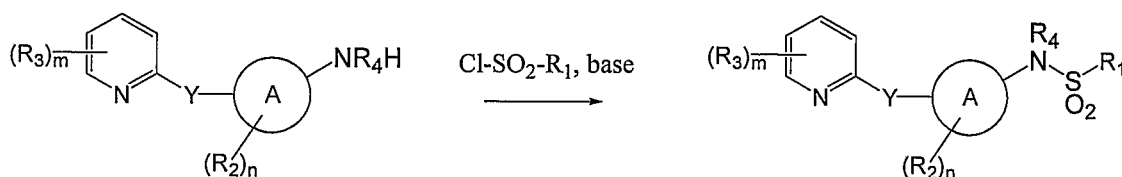
Scheme 7
