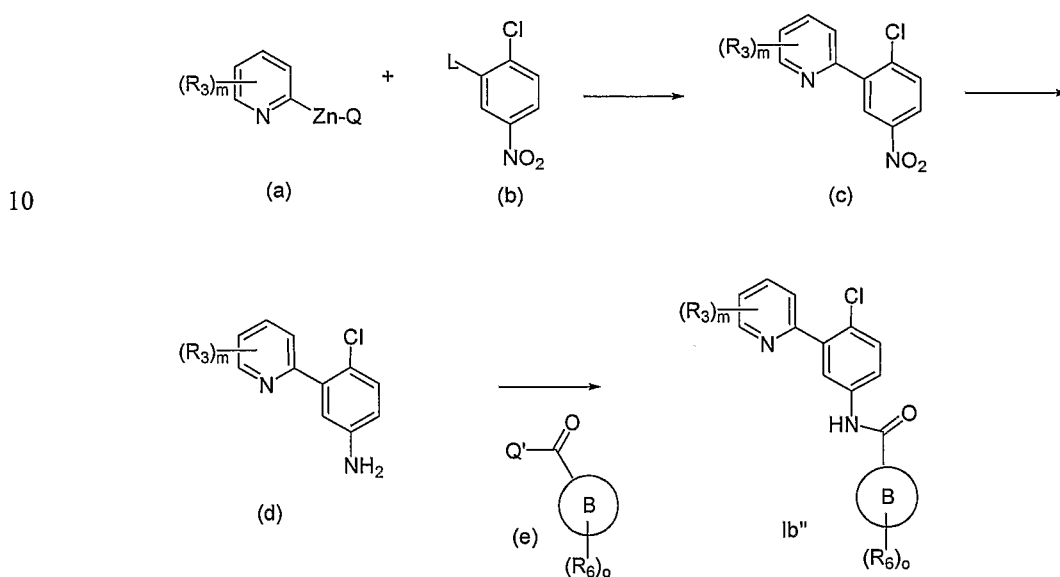
Scheme 8
