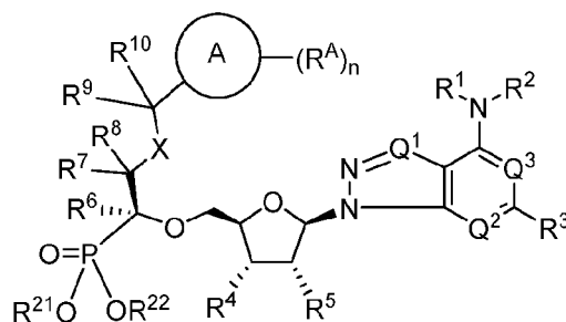
Formula (Ib).
