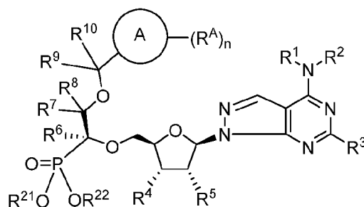
Formula (Ic).
