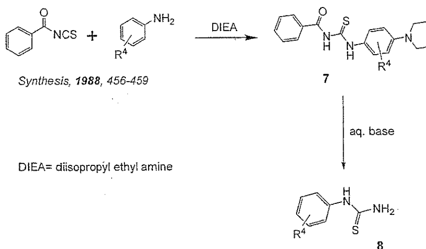
SCHEME 5
