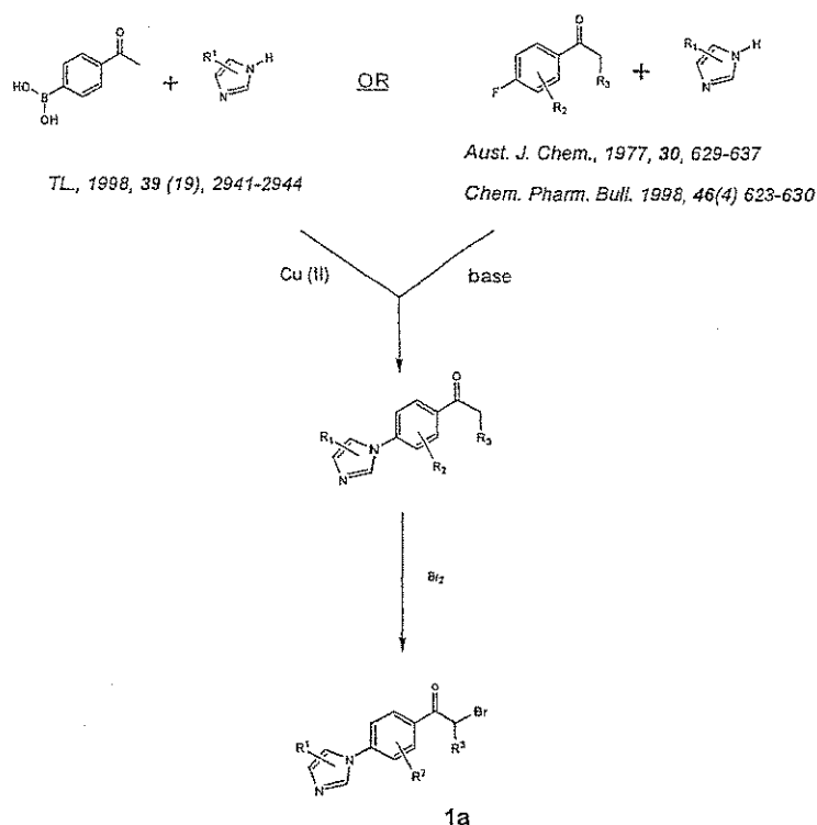
SCHEME 4
