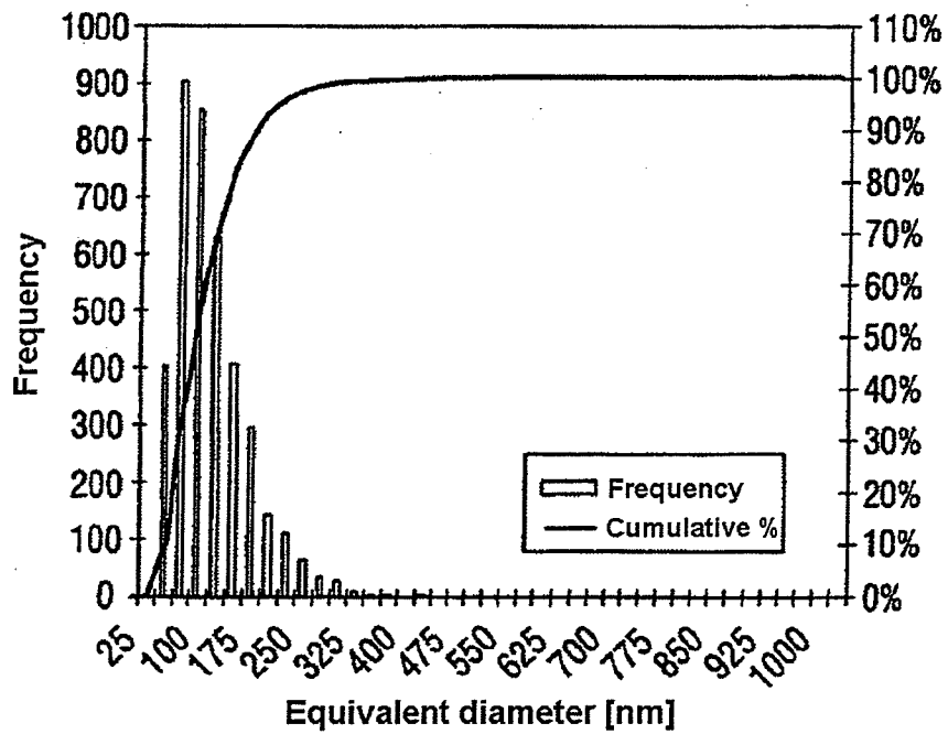
Fig. 8: Histogram of the equivalent diameters of Example 2
