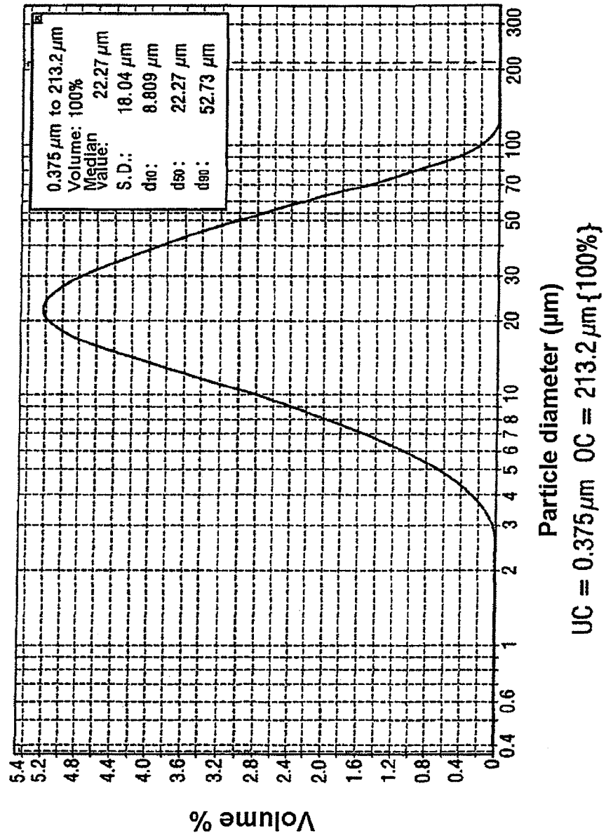
Fig. 4: Particle distribution of silica 1 (unmilled)
