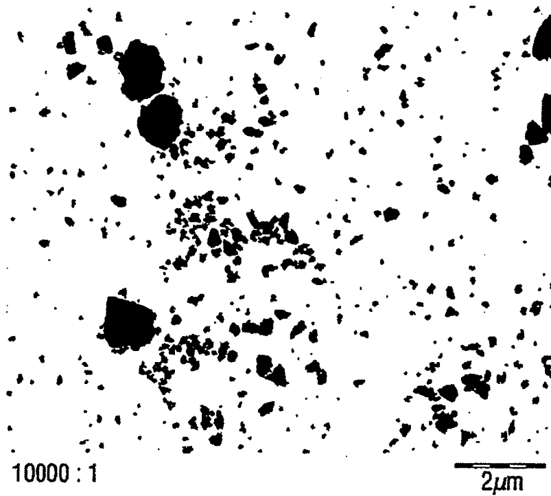
Fig. 11: Transmission electron micrograph of Example 3b
