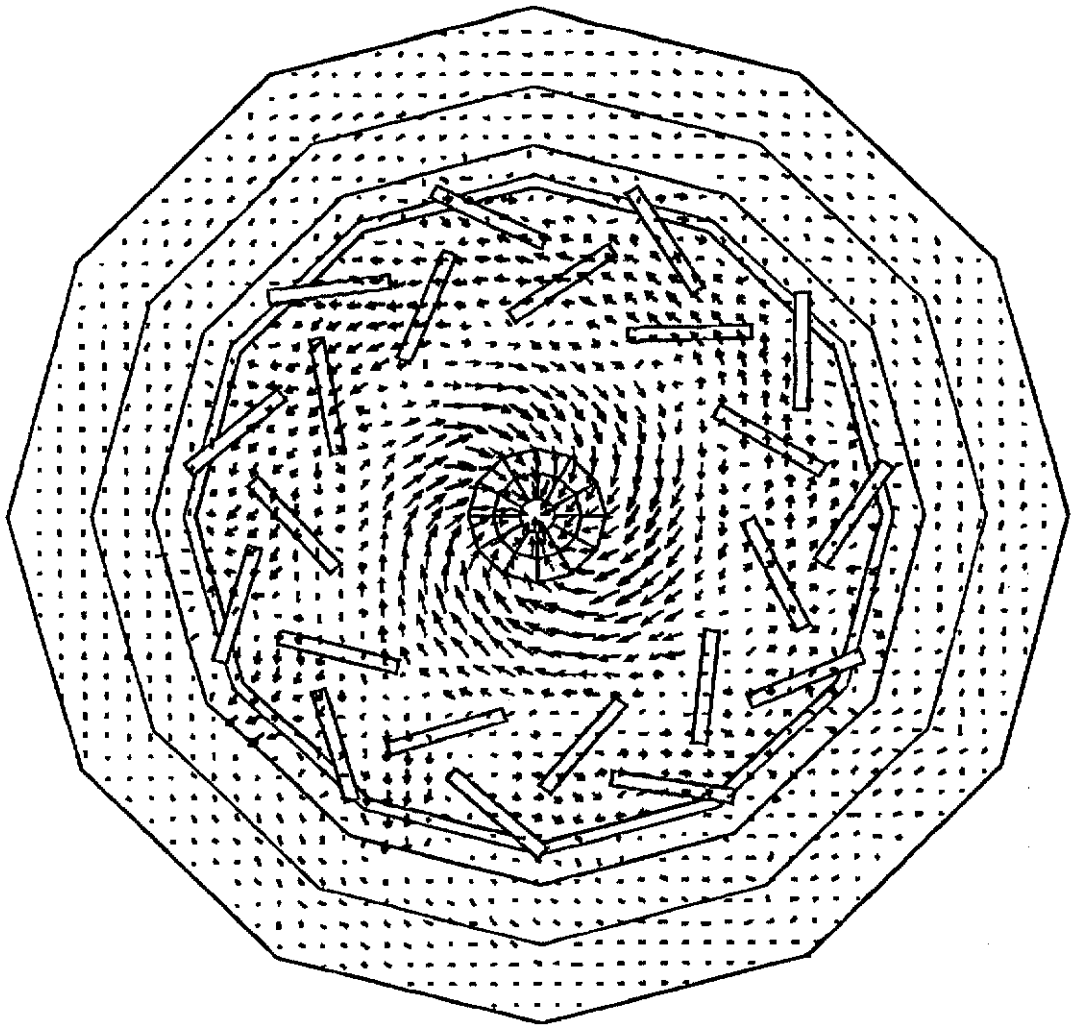
FIG. 4B ELECTRIC FIELD RIGHT BELOW MICROWAVE INTRODUCING WINDOW
