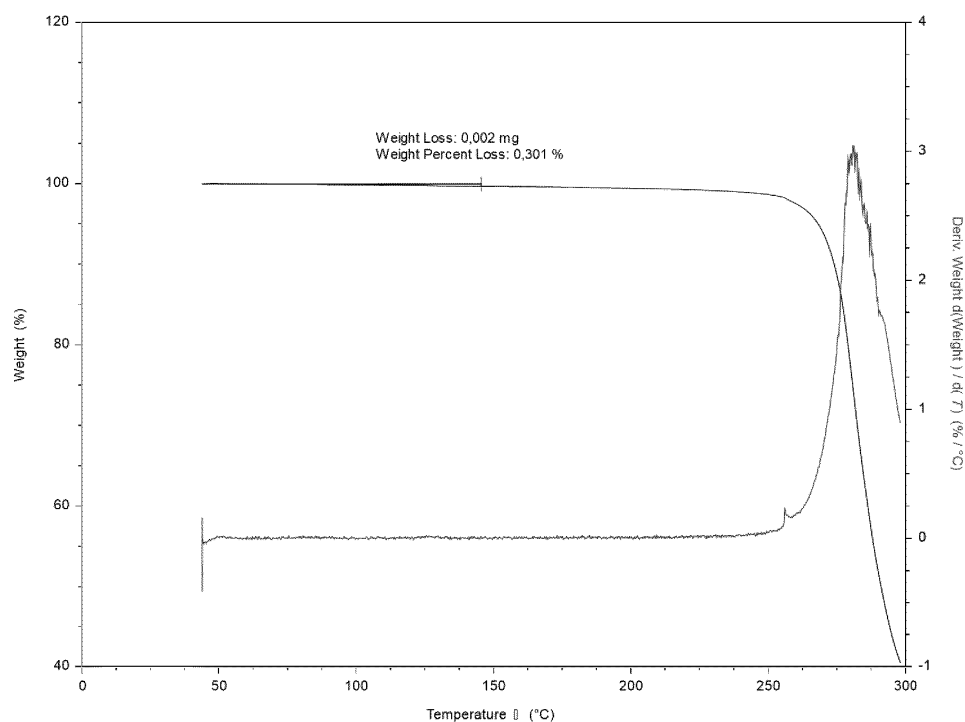
Figure 5: TGA of the crystal Form 2 of the compound of formula (I)
