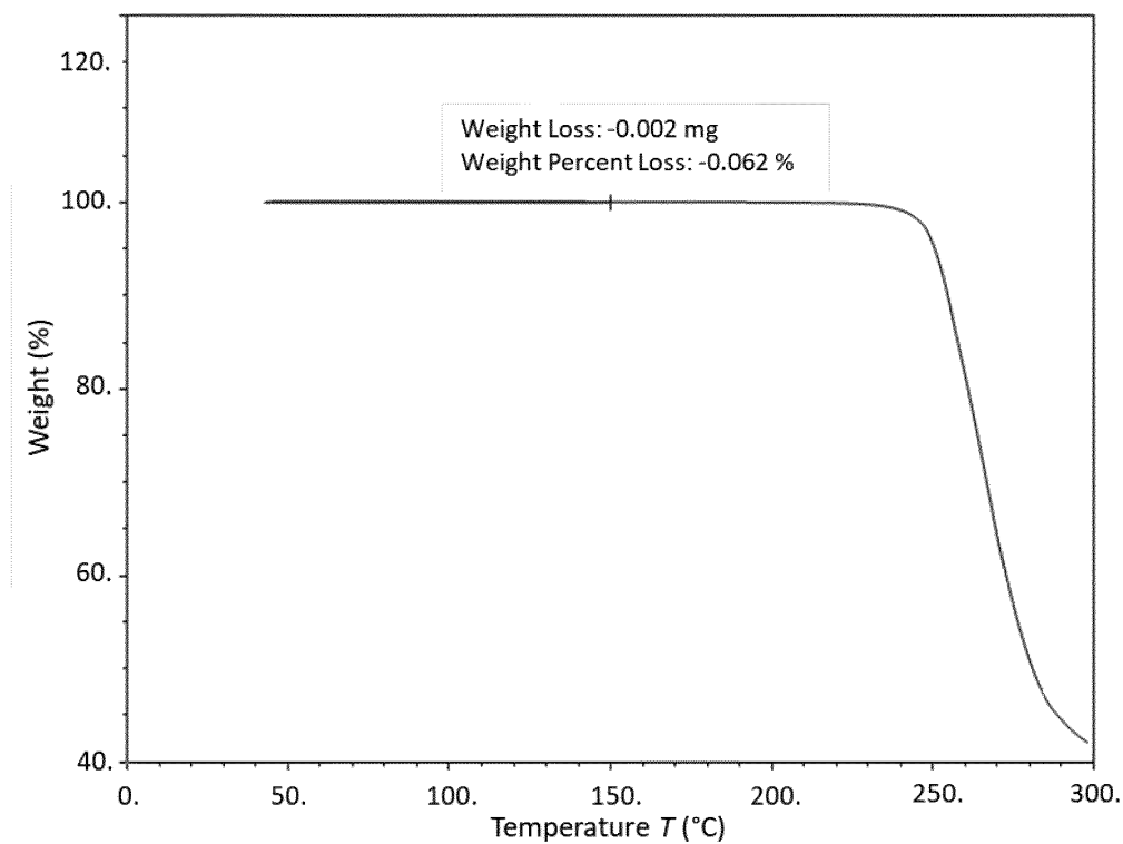
Figure 6: TGA of the crystal Form A of the compound of formula (I)
