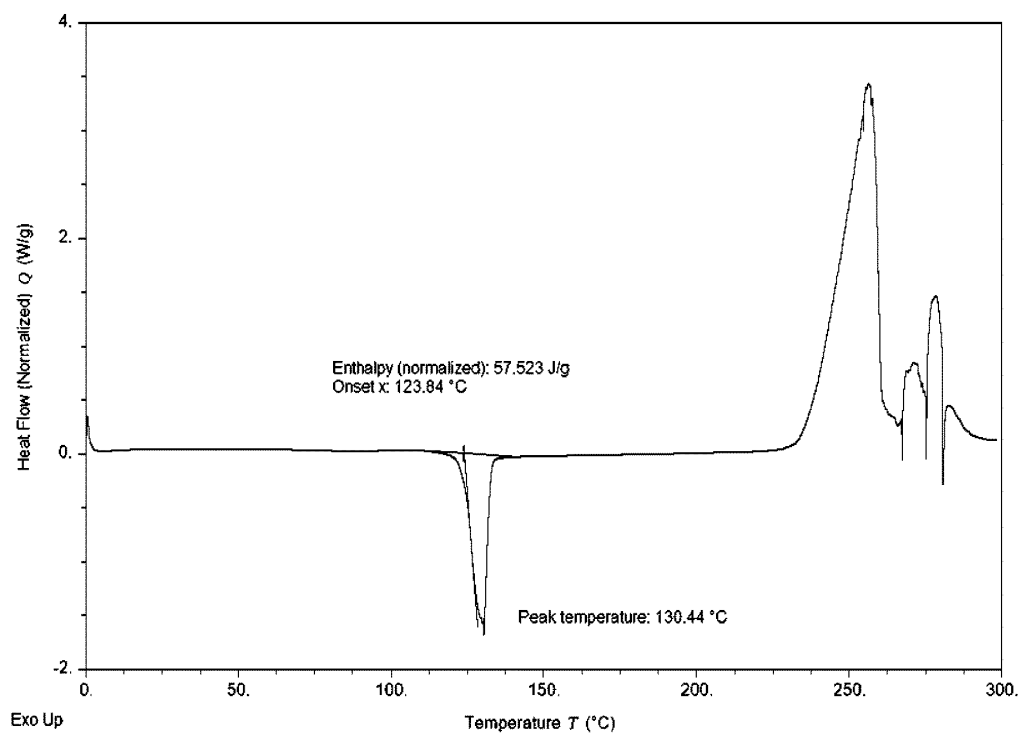
Figure 3: DSC of the crystal Form 2 of the compound of formula (I)
