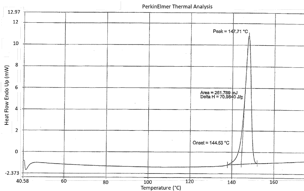
Figure 4: DSC of the crystal Form A of the compound of formula (I)
