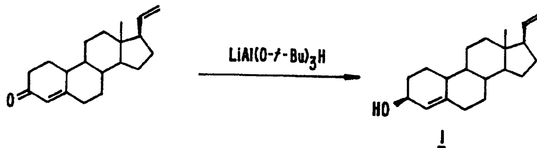
Scheme 1. Syntheses of 19-norpregnanes.
