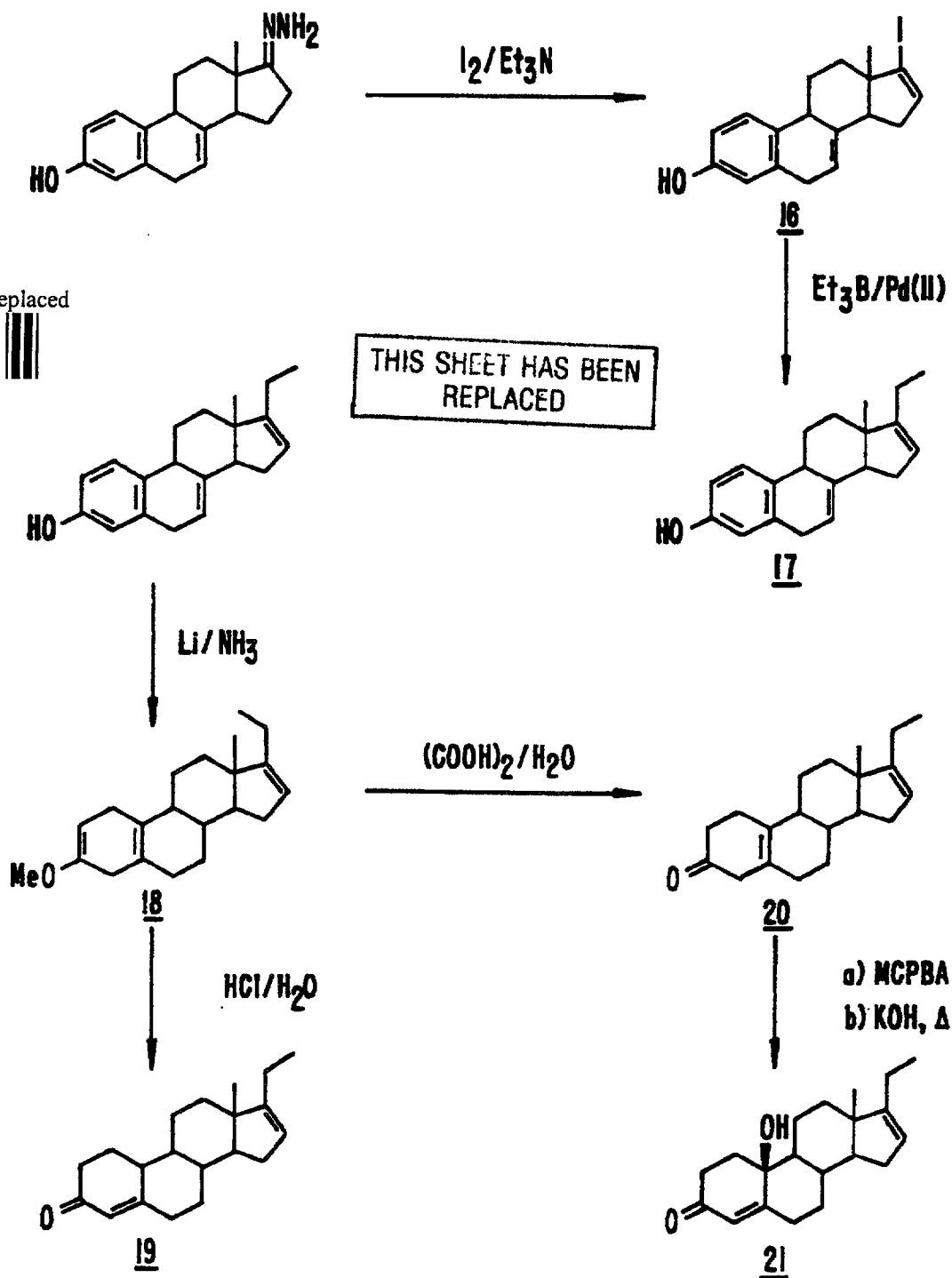
Scheme 5. Pd(II)-catalyzed synthesis of 19-norpregnenes.
