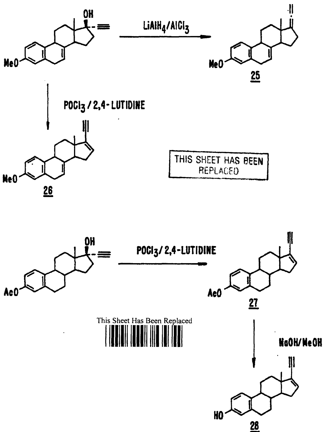
Scheme 7. Additional syntheses of 19-norpregnenes.
