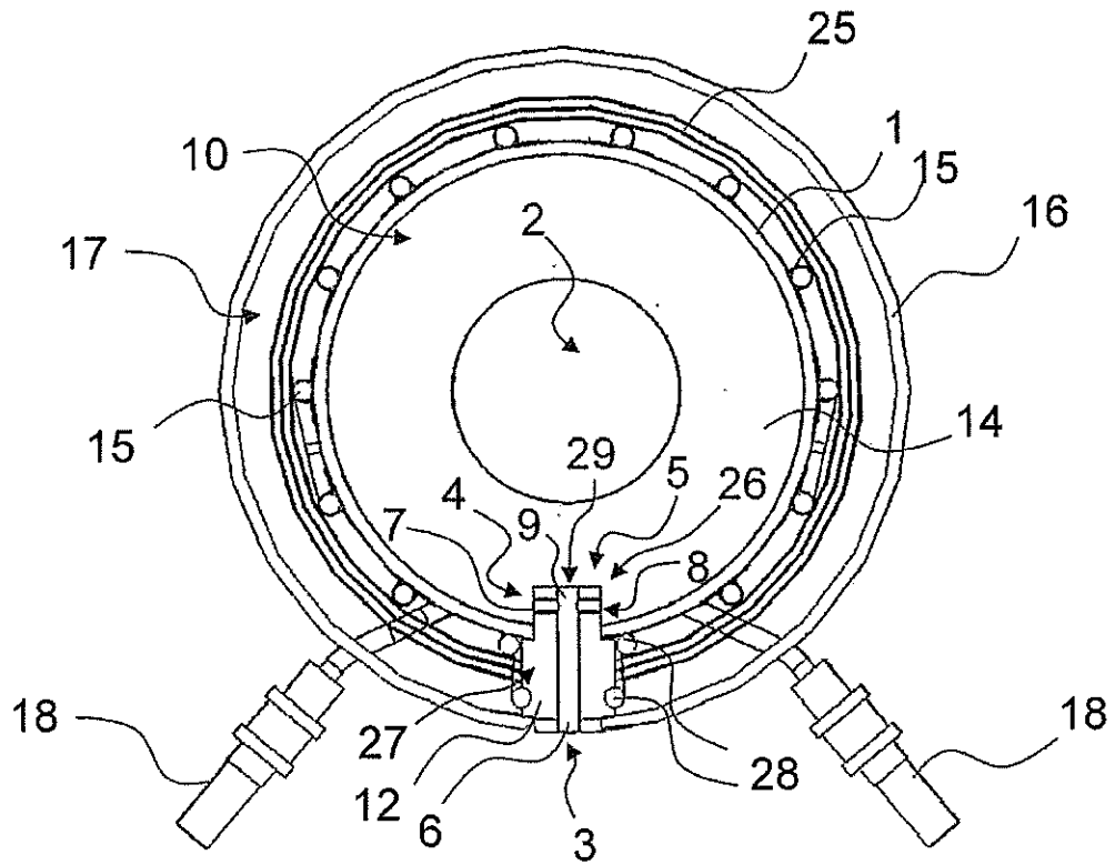
Section A-A FIGURE 3
