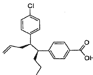
Major Diastereomer
