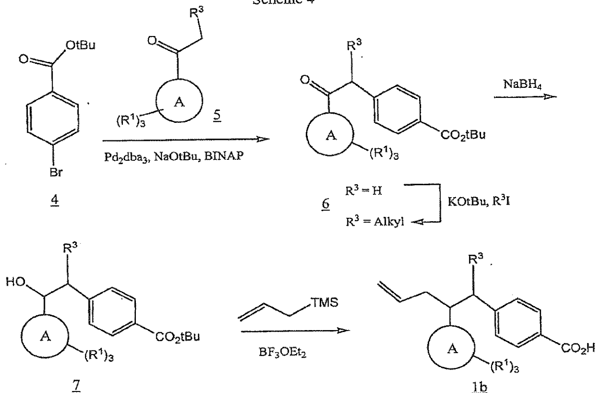
Scheme 4
