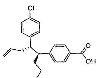
Minor Diastereomer
