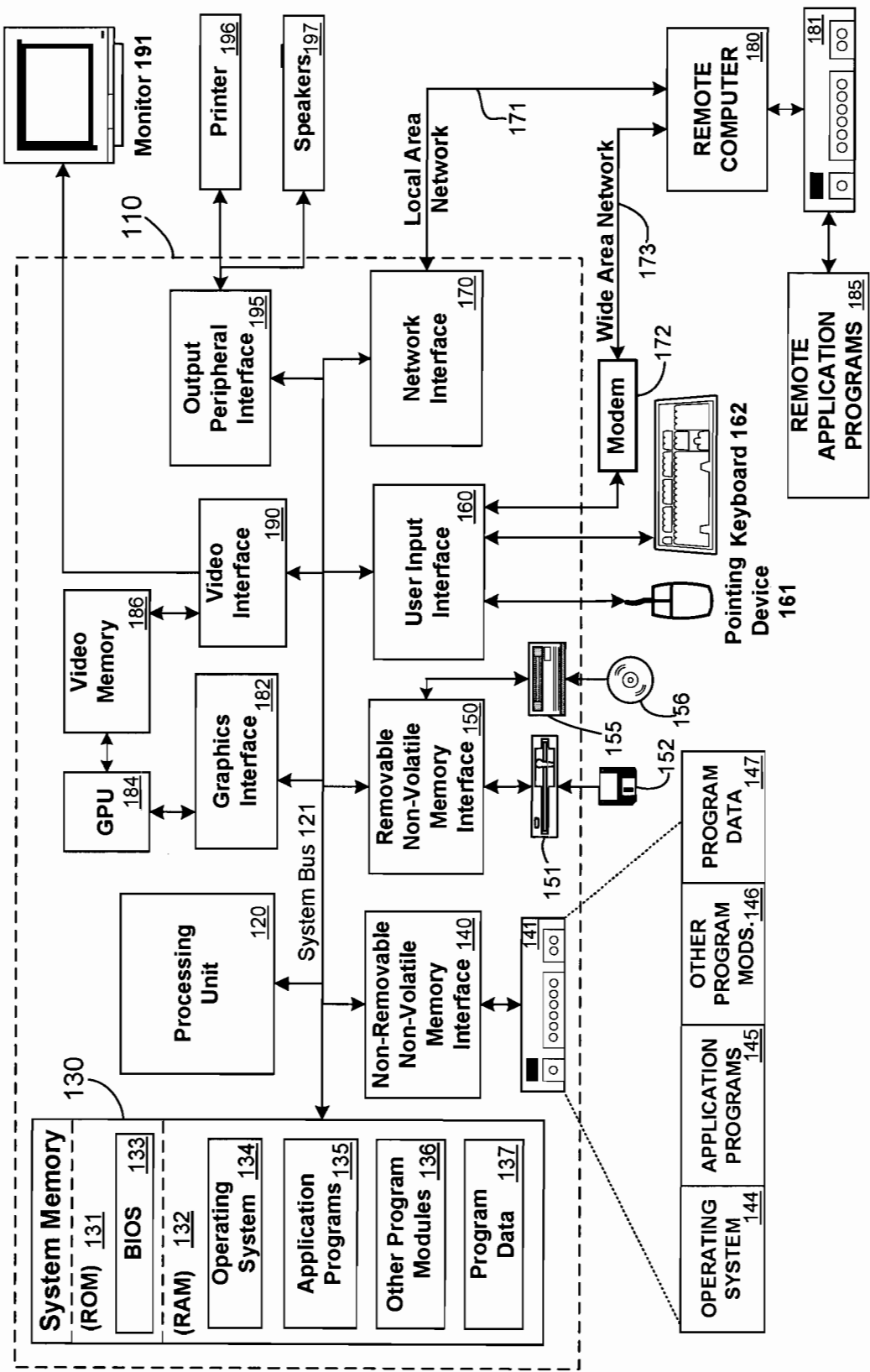
Computing Environment 100
