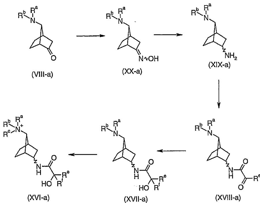
Scheme 2
