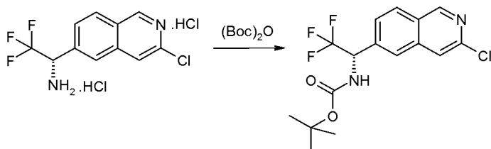
Compound 23g
