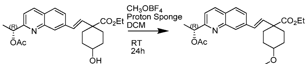
Compound 159b
