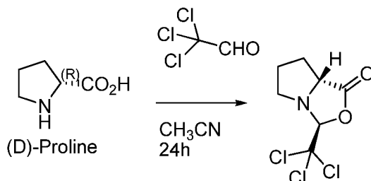
Compound 155a
