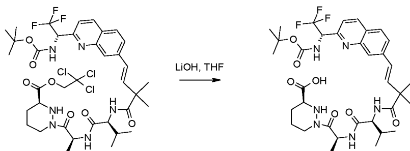
Compound 13e
