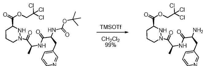
Compound 55b
