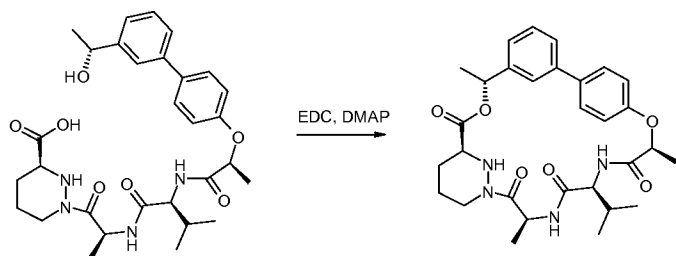
Compound 39
