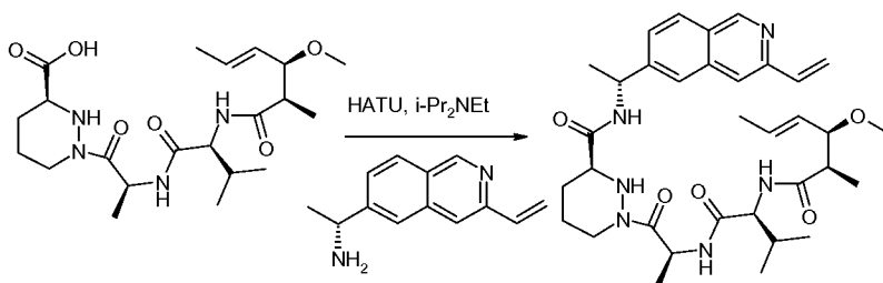
Compound 5l
