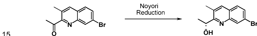
Compound 163b
