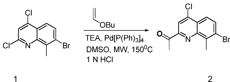
Compound 164b
