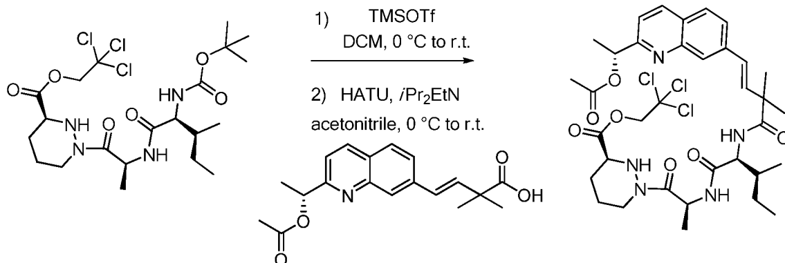
Compound 125b:
