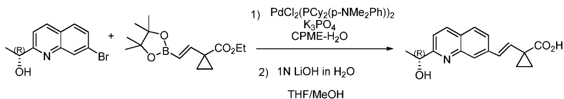
20 Compound 152a
