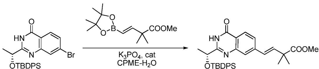
Compound 147a
