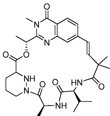
Compound 147a
