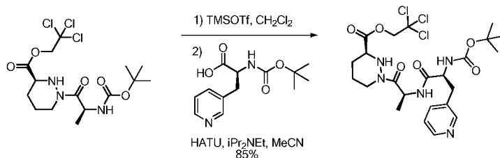
Compound 55a
