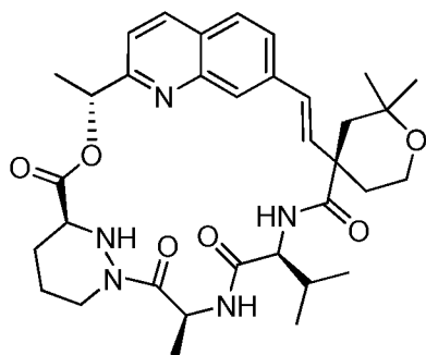
Compound 124a:
