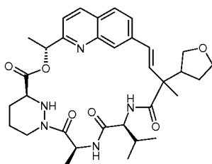
Compound 116a. (Tetrahydro-furan-3-yl)-acetic acid ethyl ester
