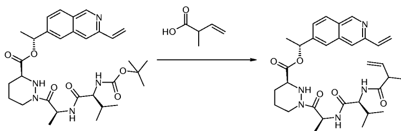
Compound 20a
