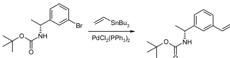
Compound 1h
