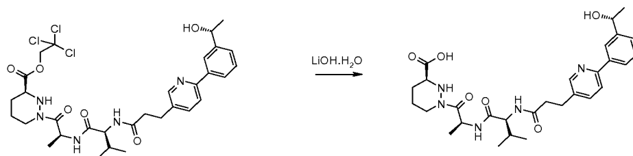
Compound 45e
