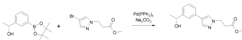
Compound 42a
