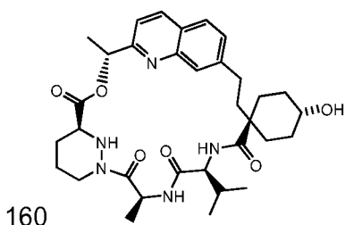
Compound 160a
