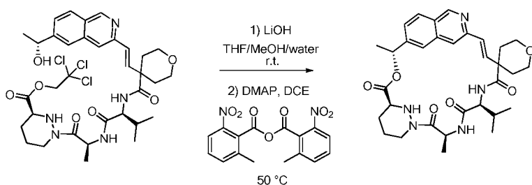
Compound 59
