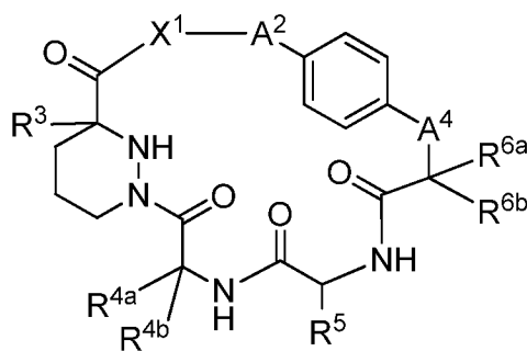
Formula IV
