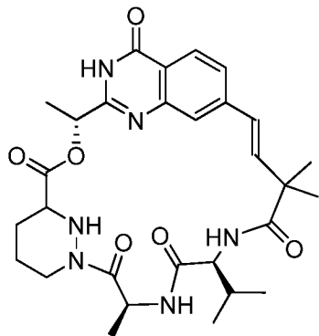
Compound 146a
