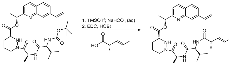
Compound 27d
