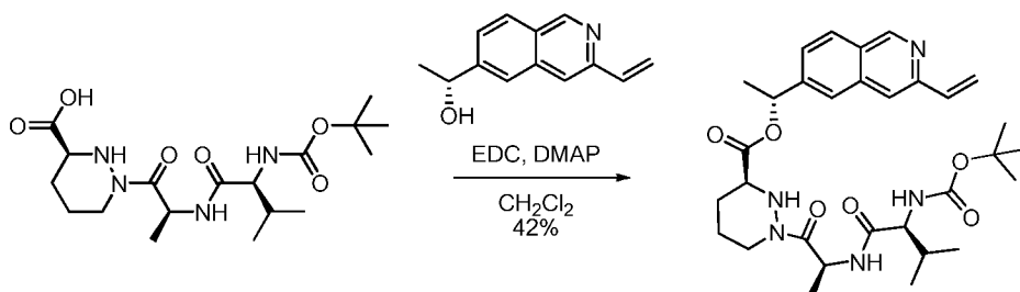
Compound 19a
