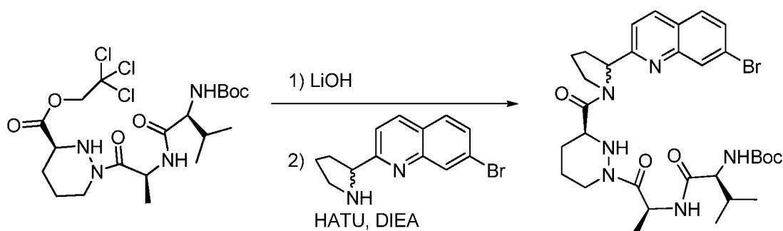
Compound 150a
