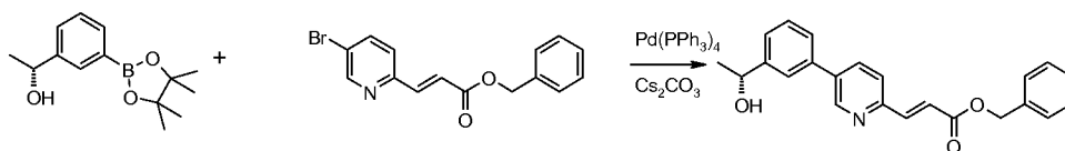
Compound 44c
