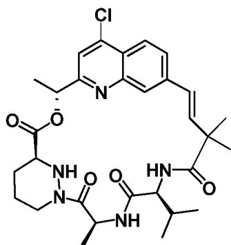
Compound 138a
