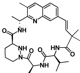
Compound 175a
