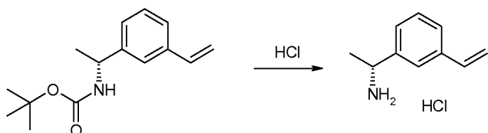
Compound 1i
