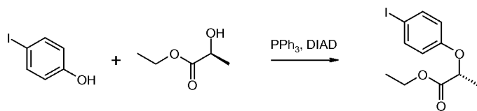
Compound 40a
