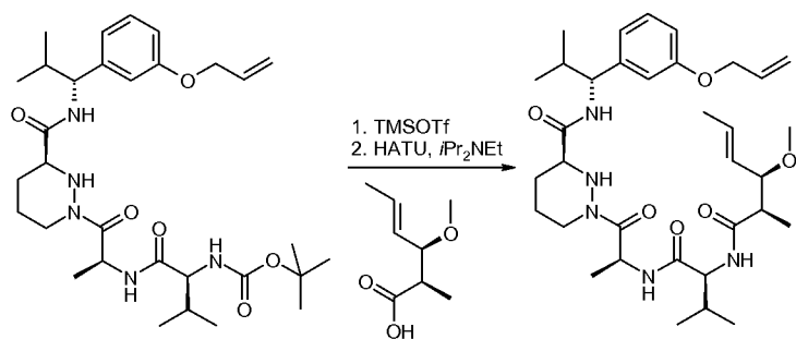
Compound 37e
