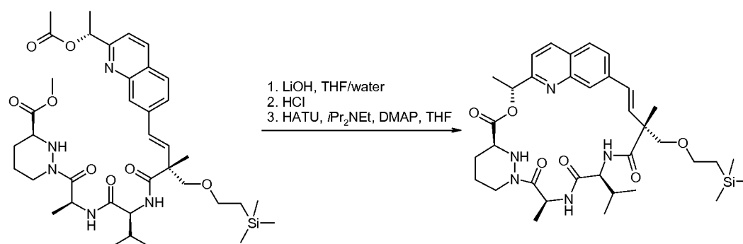
Compound 77
