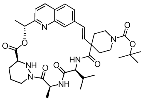
Compound 126a:
