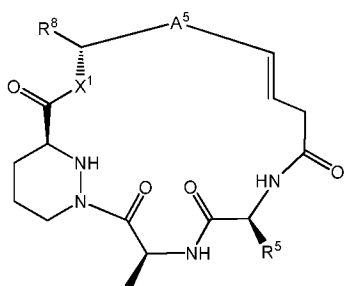
Formula (II-a)
