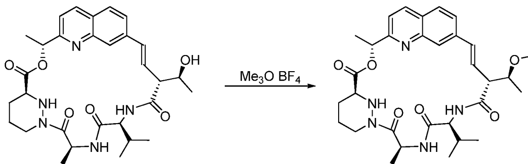
Compound 149
