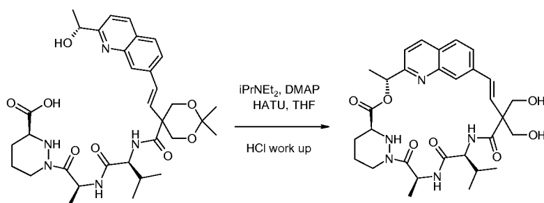
Compound 76
