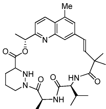
Intermediate 148a
