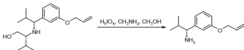
Compound 37c
