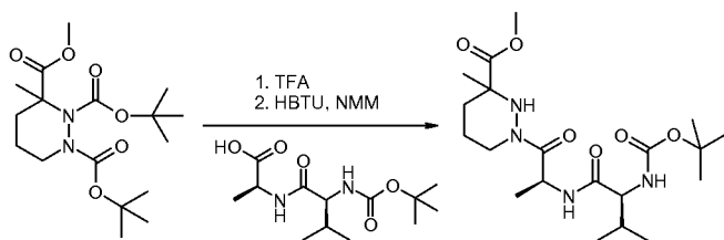
Compound 33e
