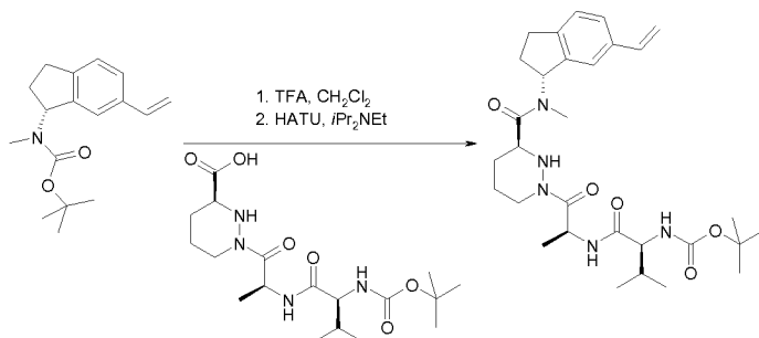
Compound 25d
