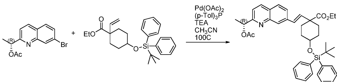
Compound 157c
