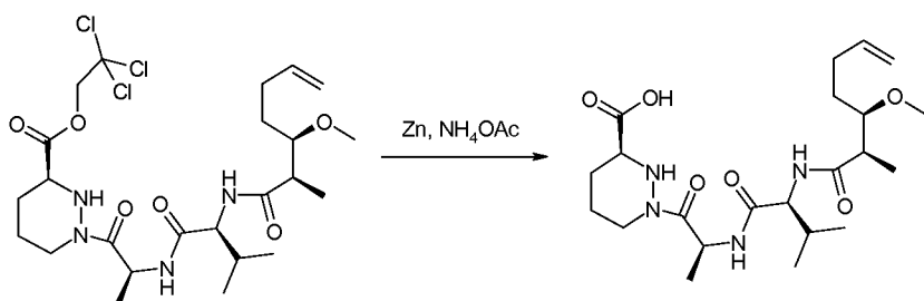
Compound 28f
