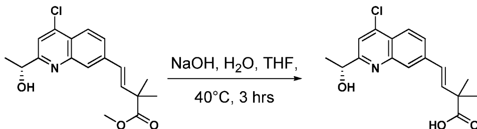
Compound 138d
