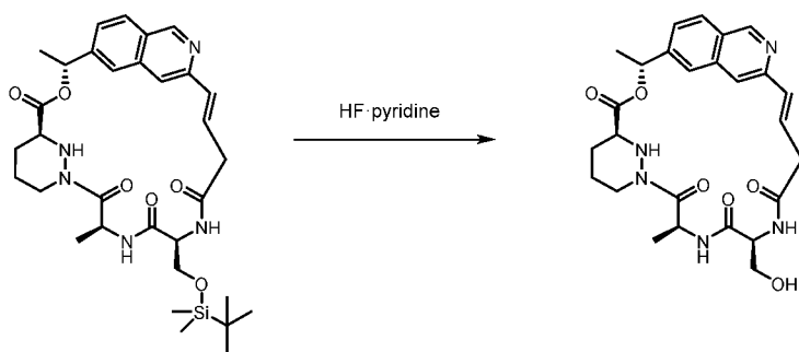
Compound 47
