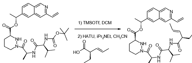
Compound 19b
