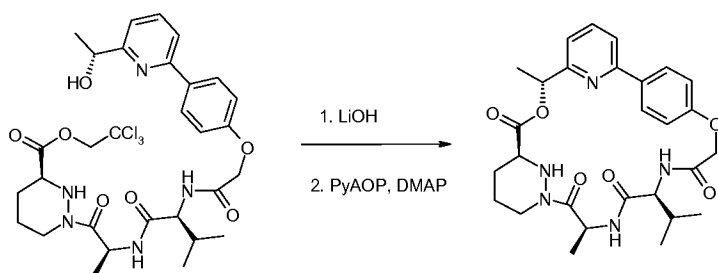
Compound 41
