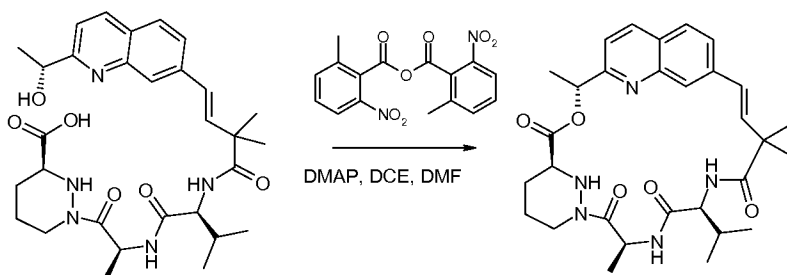
Compound 22
