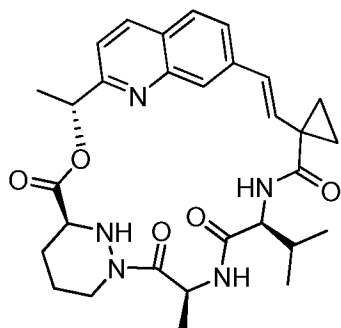
20 Compound 152a
