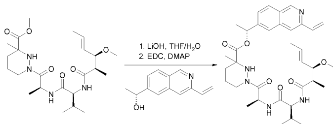
Compound 33g
