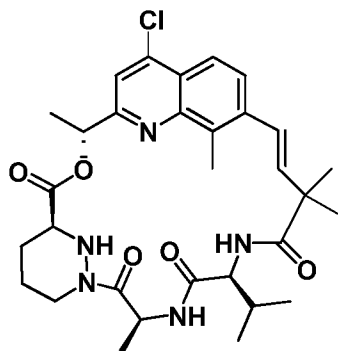
Compound 164a
