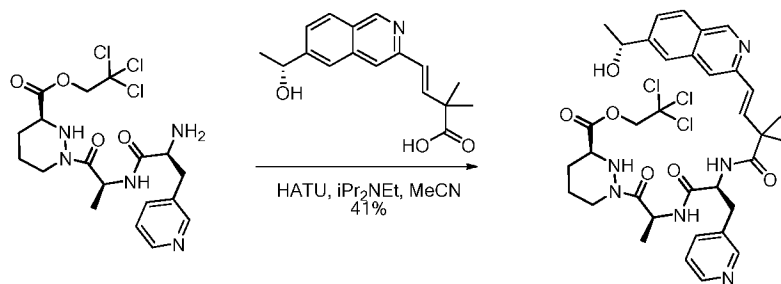
Compound 55c
