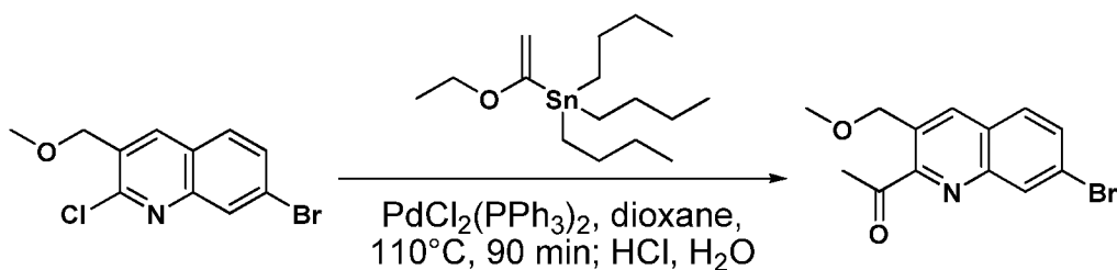
Compound 137b
