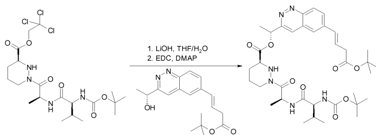
Compound 32h
