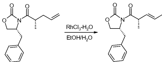
Compound 27b
