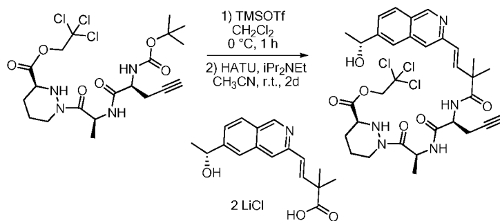
Compound 51b
