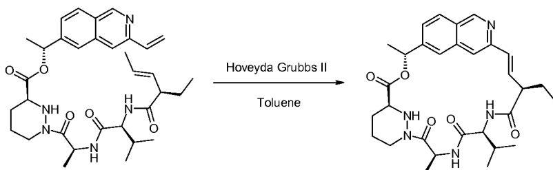
Compound 19
