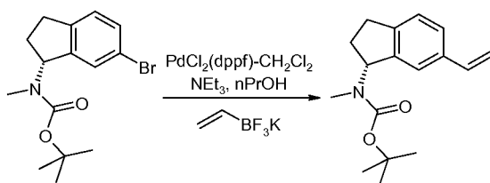
Compound 25c
