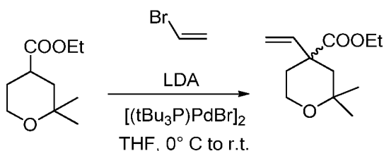
Compound 124a:
