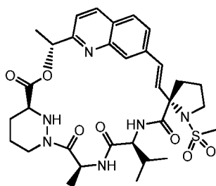
Compound 156a
