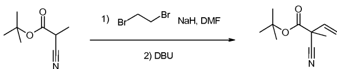
Compound 85a: 2-Cyano-2-methyl-but-3-enoic acid tert -butyl ester
