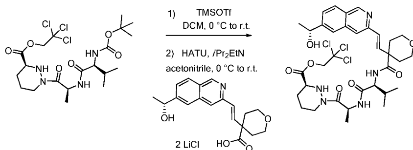
Compound 59g
