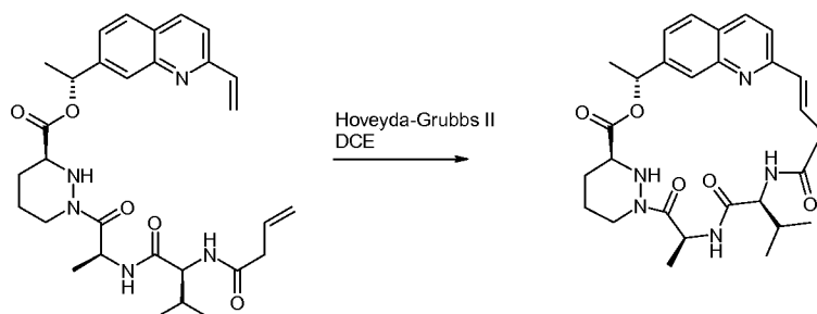
Compound 16
