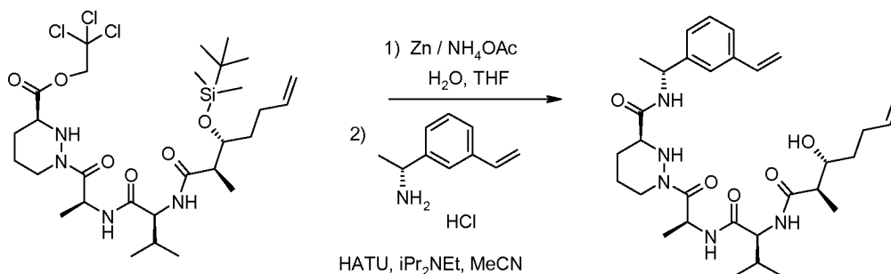
Compound 1j
