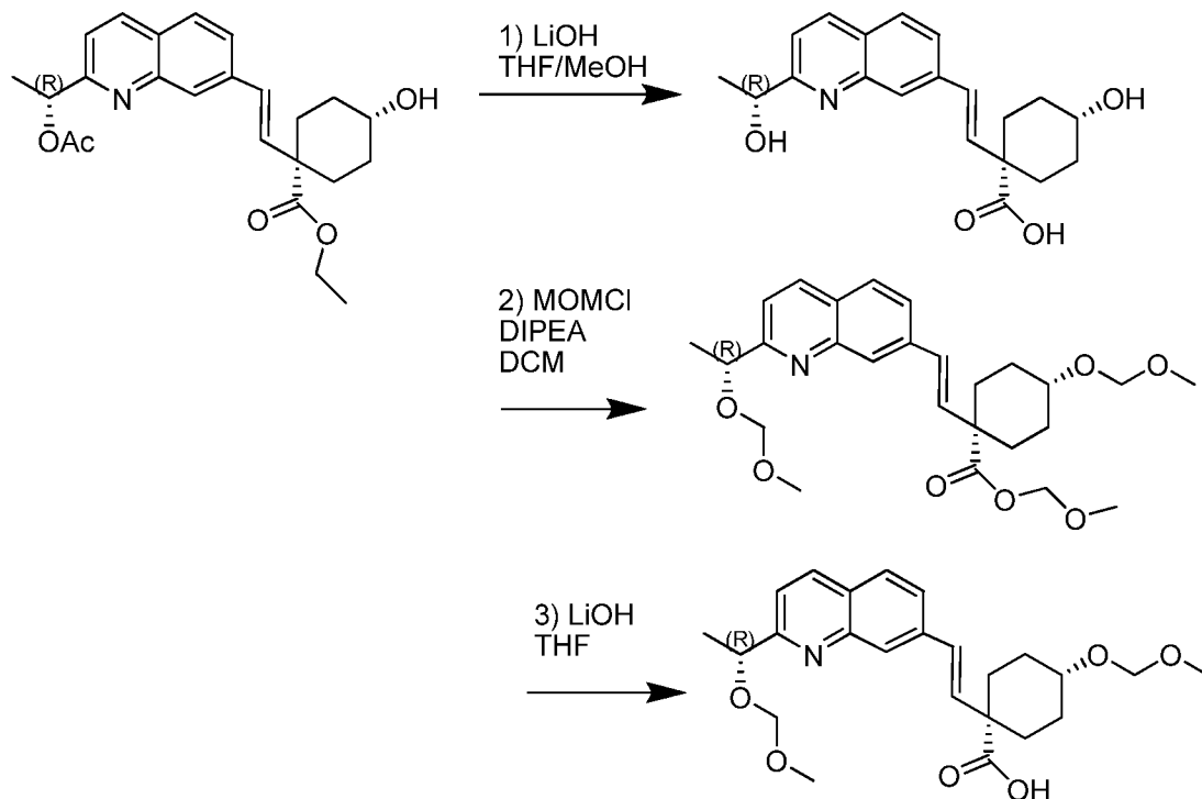
Compound 160d
