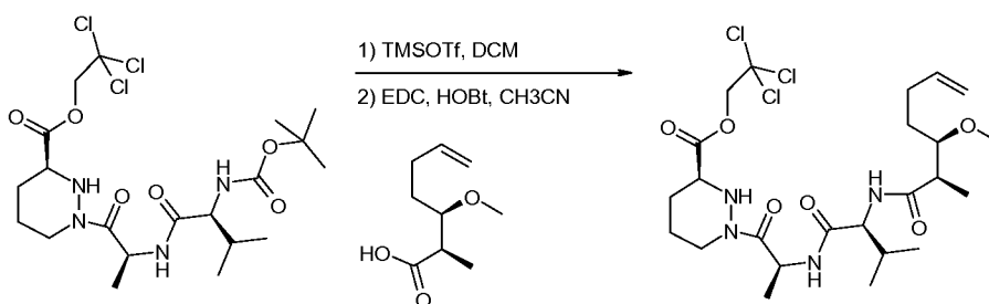
Compound 28e
