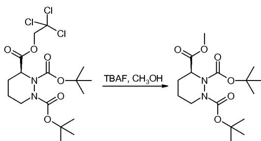
Compound 33a
