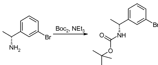
Compound 1g
