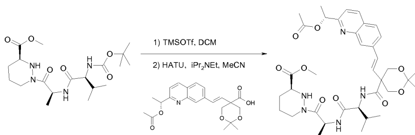
Compound 75g
