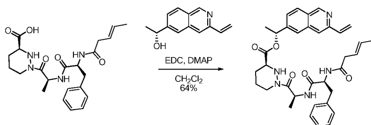
Compound 54d
