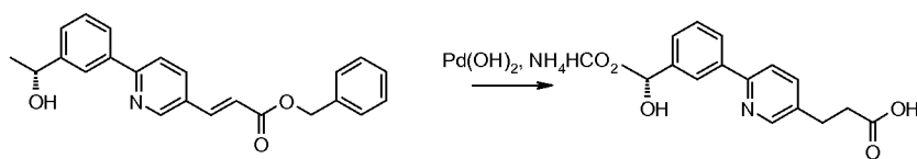
Compound 45c
