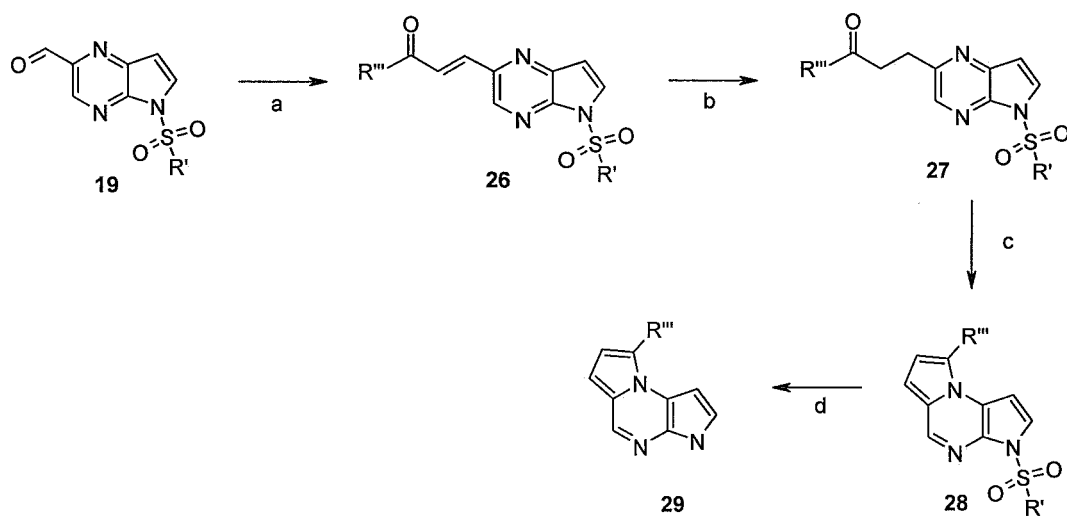
Scheme V
