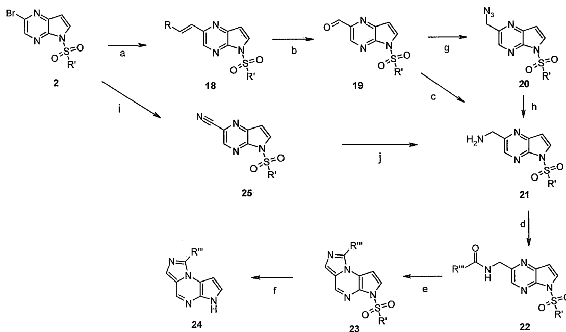
Scheme IV
