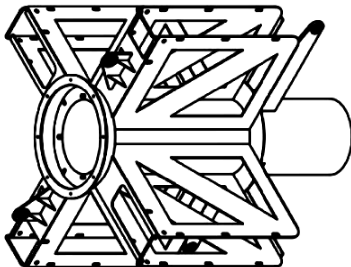
ISO VIEW
