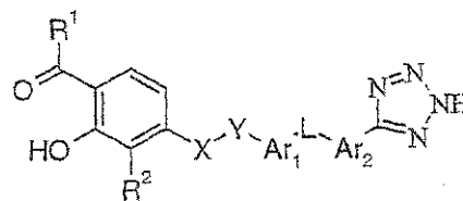
tautomer II
