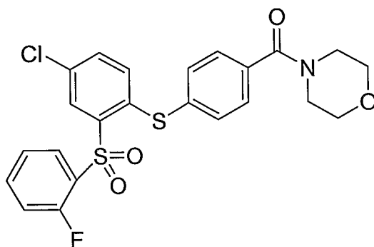
Compound XXVII
