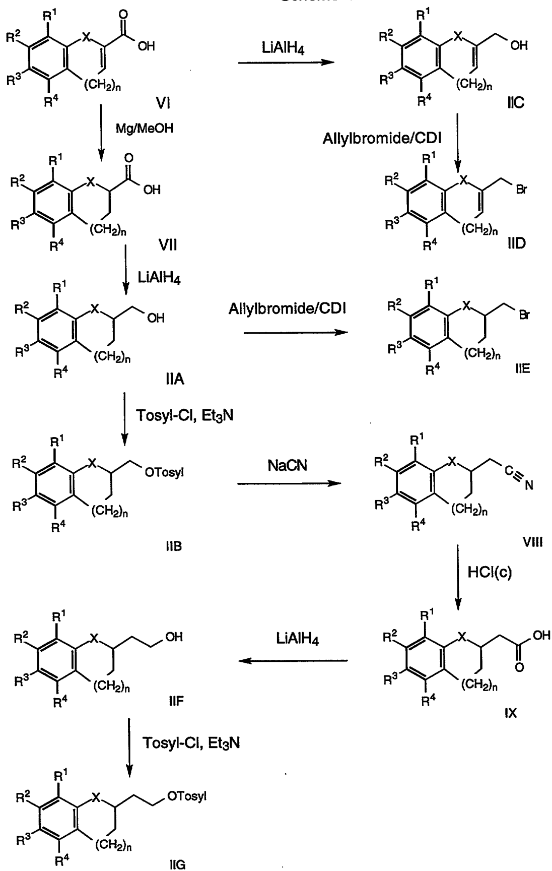
Scheme 1
