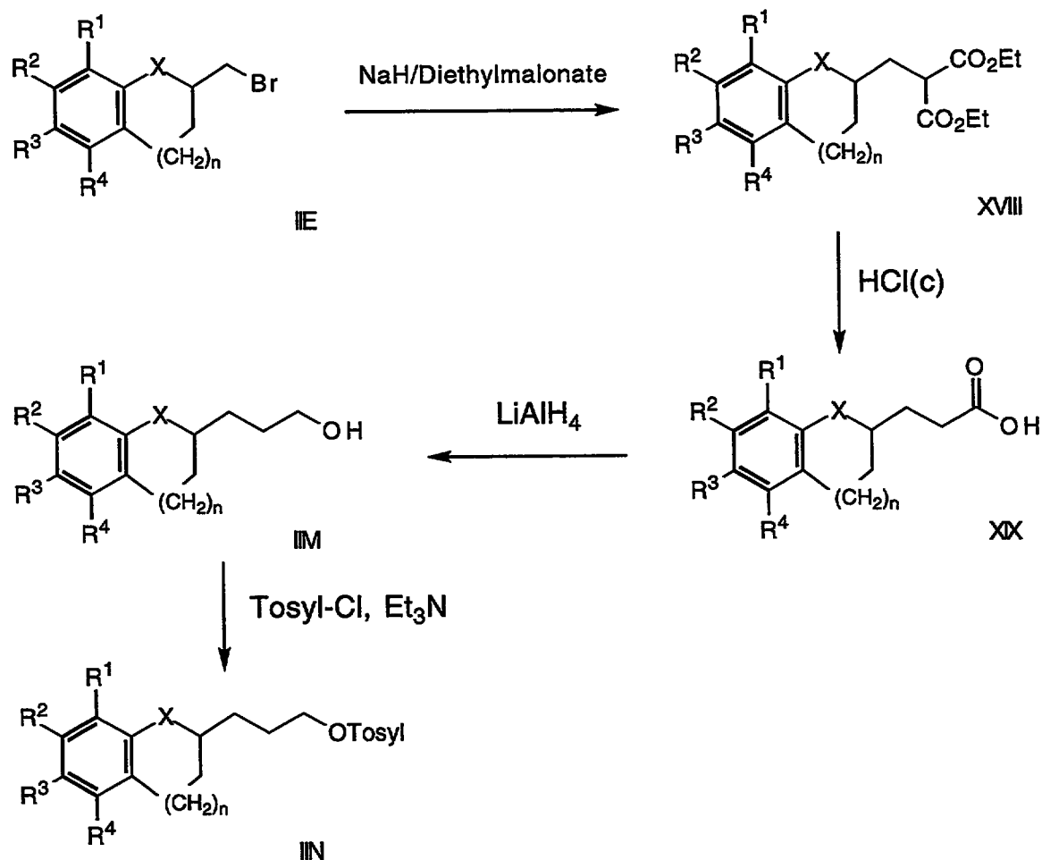
Scheme 5
