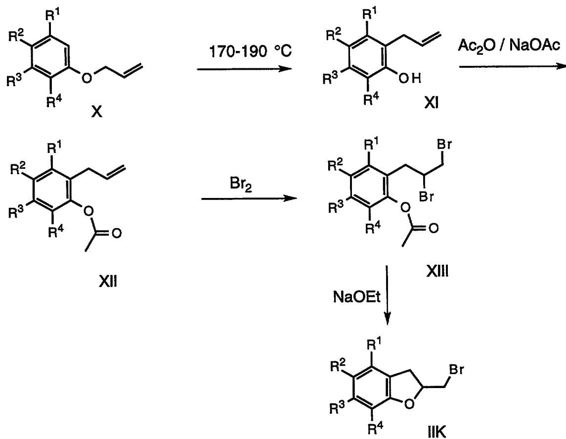
Scheme 3
