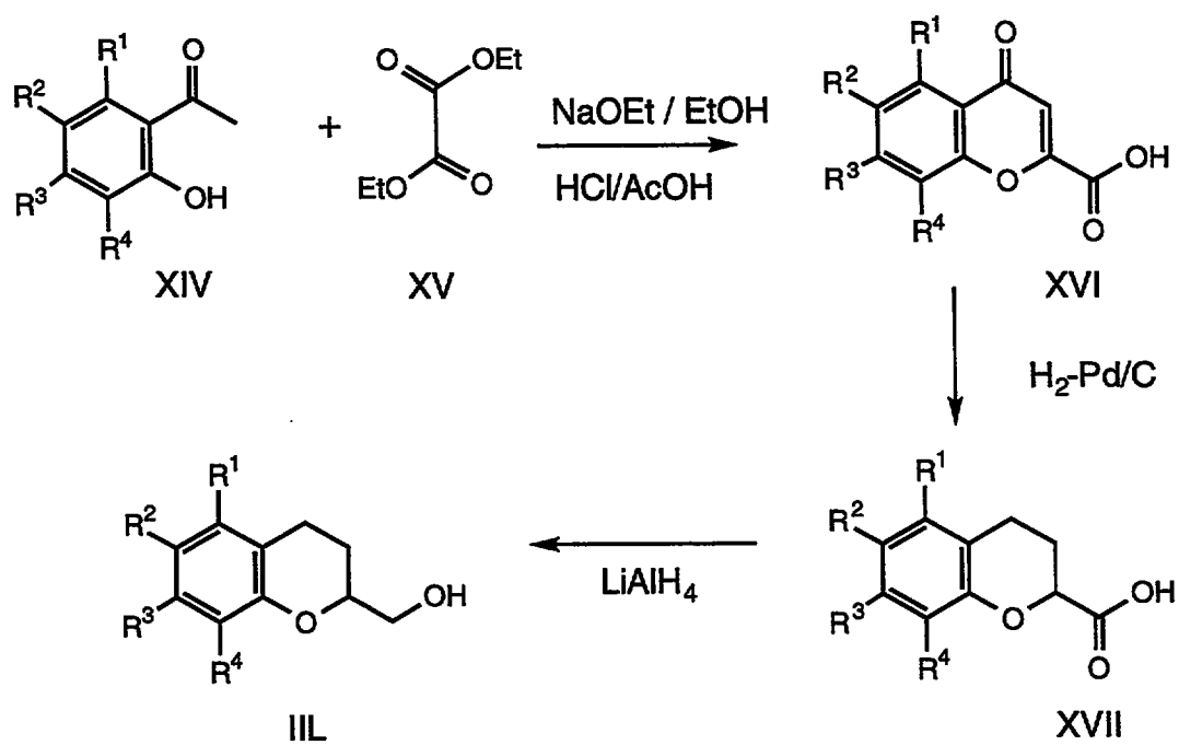
Scheme 4
