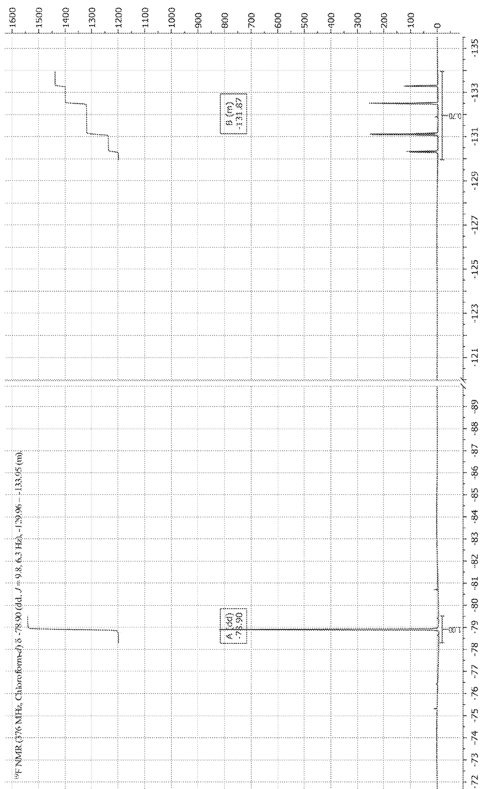
Figure 2a: Proton decoupled ^{19}\text{F} NMR spectrum
