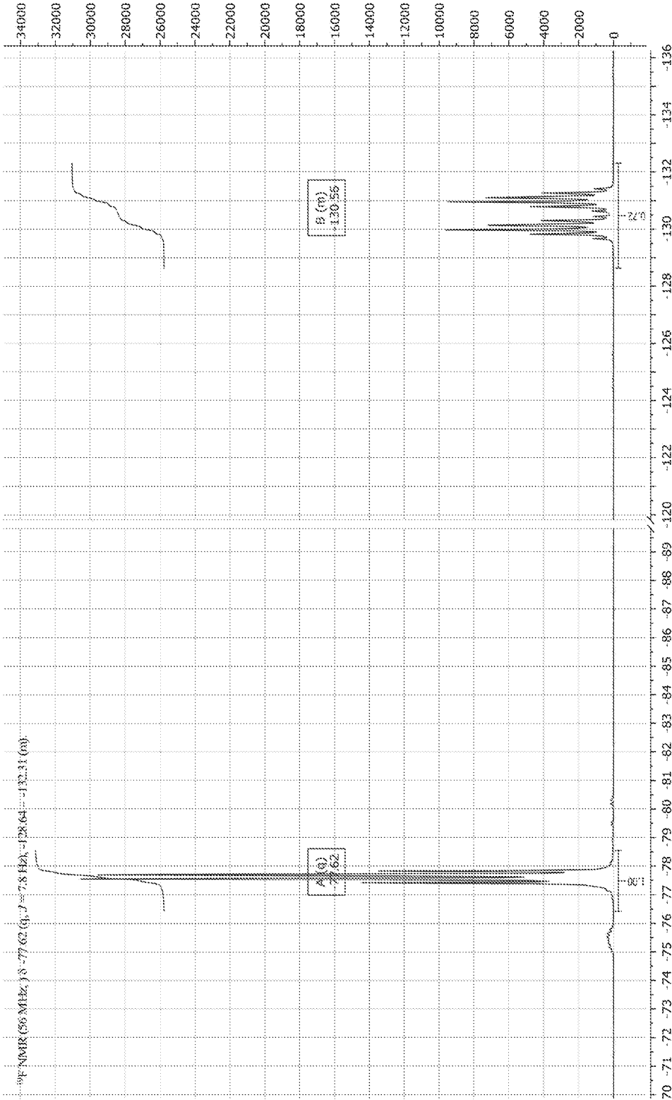
Figure 2a: Proton coupled 19 F NMR spectrum
