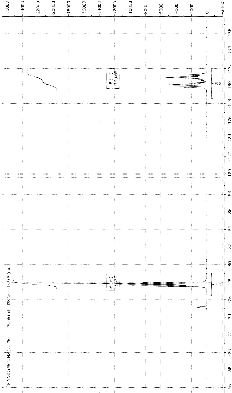
Figure 2: Proton coupled 19 F NMR spectrum
