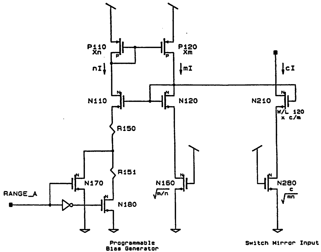
Figure 3 Programmable Reference Generator With MOS Switching
