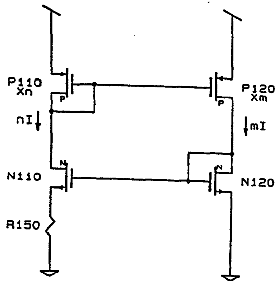
Figure 1 Bias Generator (Prior Art)
