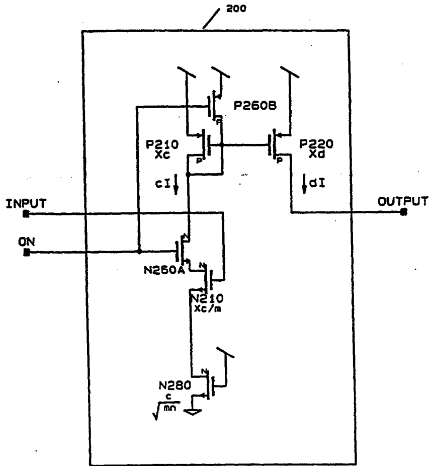
Figure 6(a) Switch Mirror Current Gain = d/c
