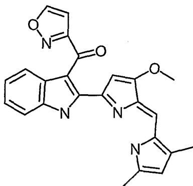
Compound 23 {2-[5-(3,5-Dimethyl-1H-pyrrol-2-ylmethylene)-4-methoxy-5H-pyrrol-2-yl]-1H-indol-3-yl}-isoxazol-3-yl-methanone;
