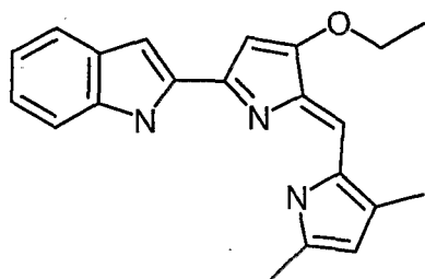
Compound 28 2-[5-(3,5-Dimethyl-1H-pyrrol-2-ylmethylene)-4-ethoxy-5H-pyrrol-2-yl]-1H-indole;
