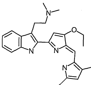
Compound 31 (2-{2-[5-(3,5-Dimethyl-1H-pyrrol-2-ylmethylene)-4-ethoxy-5H-pyrrol-2-yl]-1H-indol-3-yl}-ethyl)-dimethyl-amine;
