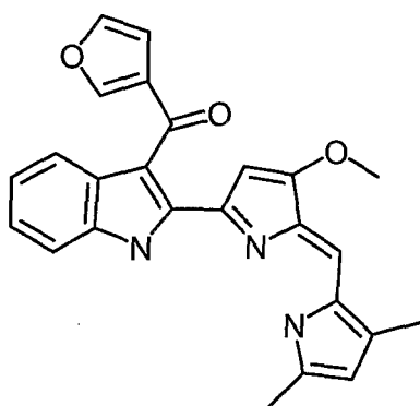
Compound 27 {2-[5-(3,5-Dimethyl-1H-pyrrol-2-ylmethylene)-4-methoxy-5H-pyrrol-2-yl]-1H-indol-3-yl}-furan-3-yl-methanone;
