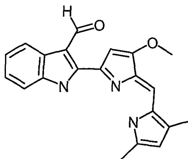
Compound 26 2-[5-(3,5-Dimethyl-1H-pyrrol-2-ylmethylene)-4-methoxy-5H-pyrrol-2-yl]-1H-indole-3-carbaldehyde;
