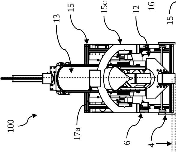
Figure 3F Front View
