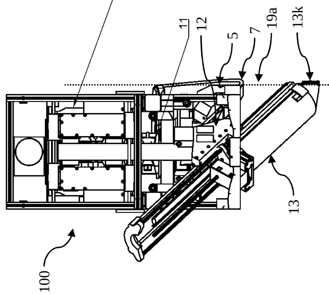
Figure 2C Top View
