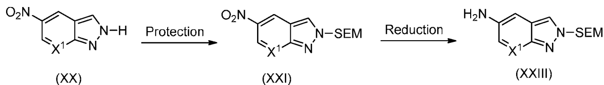
SCHEME 6
