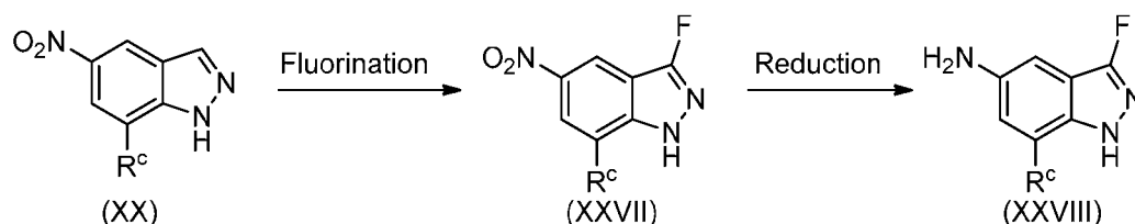
SCHEME 9
