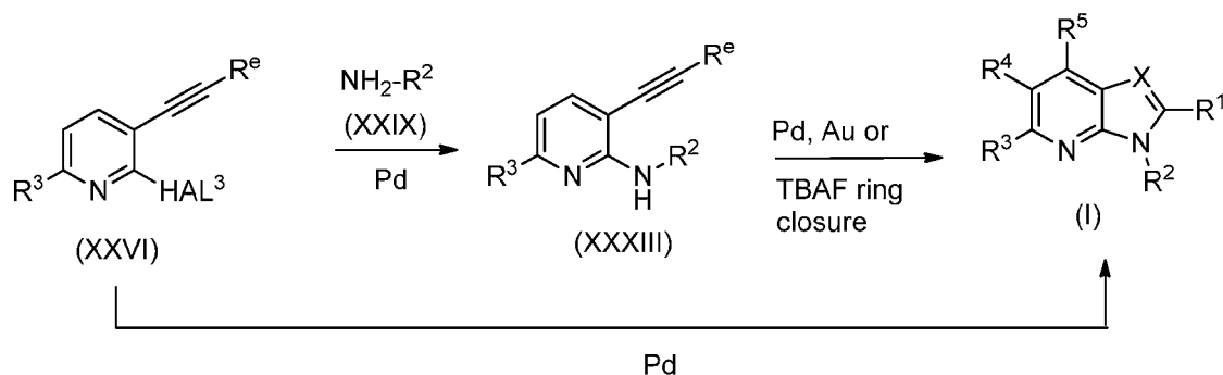
SCHEME 16
