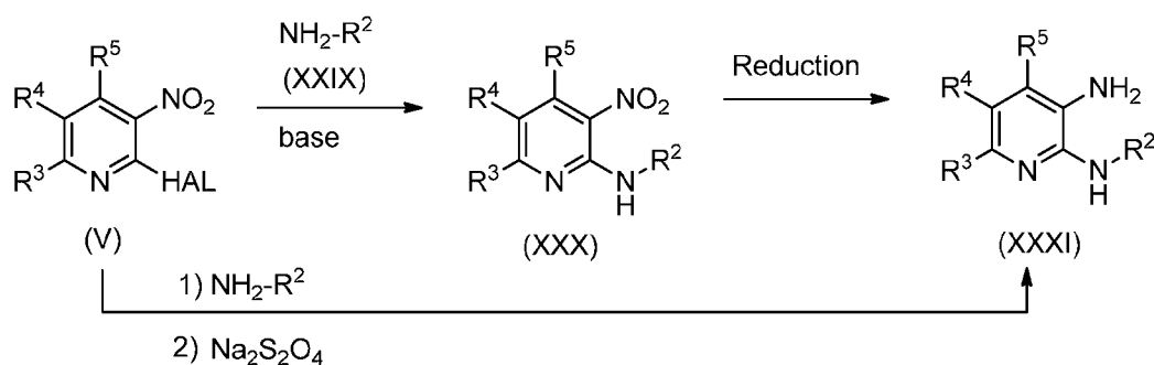
SCHEME 10
