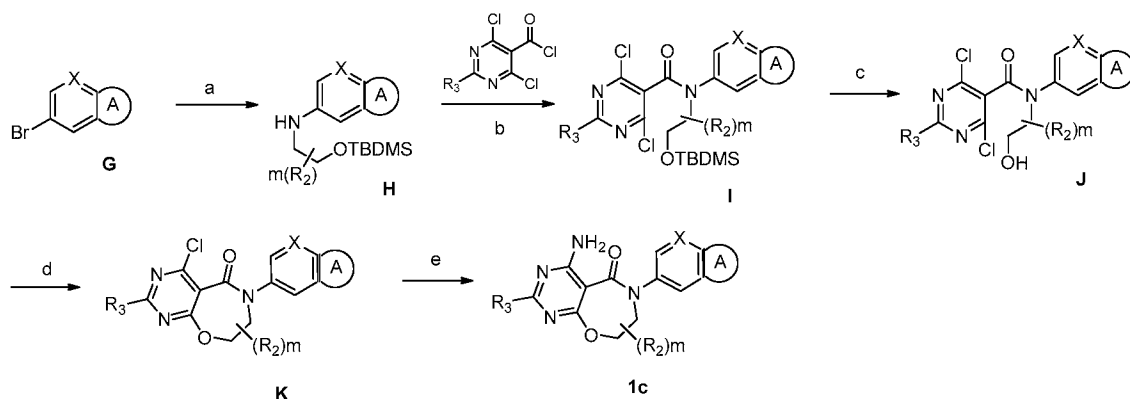
Scheme 2. Reagents and conditions: a) \text{NH}_2(\text{CH}_2)_2\text{OTBDMS} , \text{Pd}(\text{OAc})_2 , \text{Cs}_2\text{CO}_3 , X-PHOS, Toluene, 120^\circ\text{C} ; b) THF, \text{Et}_3\text{N} , RT; c) 3% HCl-MeOH, RT; d) \text{CH}_3\text{CN} , \text{Et}_3\text{N} , 80^\circ\text{C} ; e) \text{NH}_3 , Dioxane, RT.
