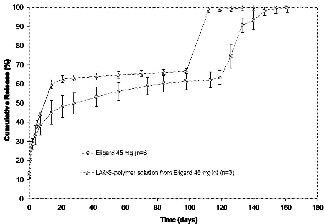
Figure 4: LAMS release from Eligard® 45mg polymer solution compared with Eligard® 45 mg release
