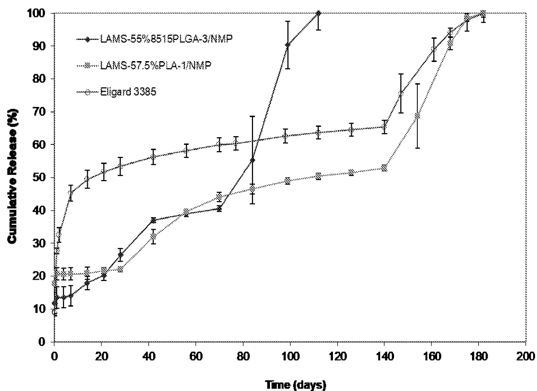
Figure 1: In vitro release of leuprolide mesylate from different polymers compared with Eligard® 45 mg release
