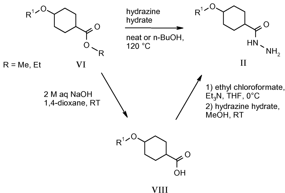
Scheme 7: General Scheme G
