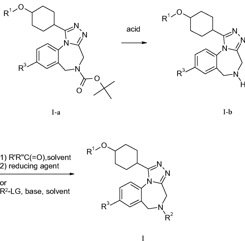
Scheme 2: General Scheme B
