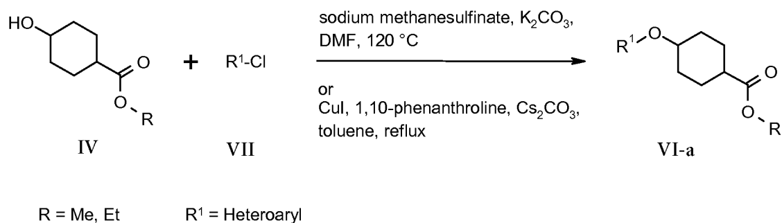
Scheme 5: General Scheme E
