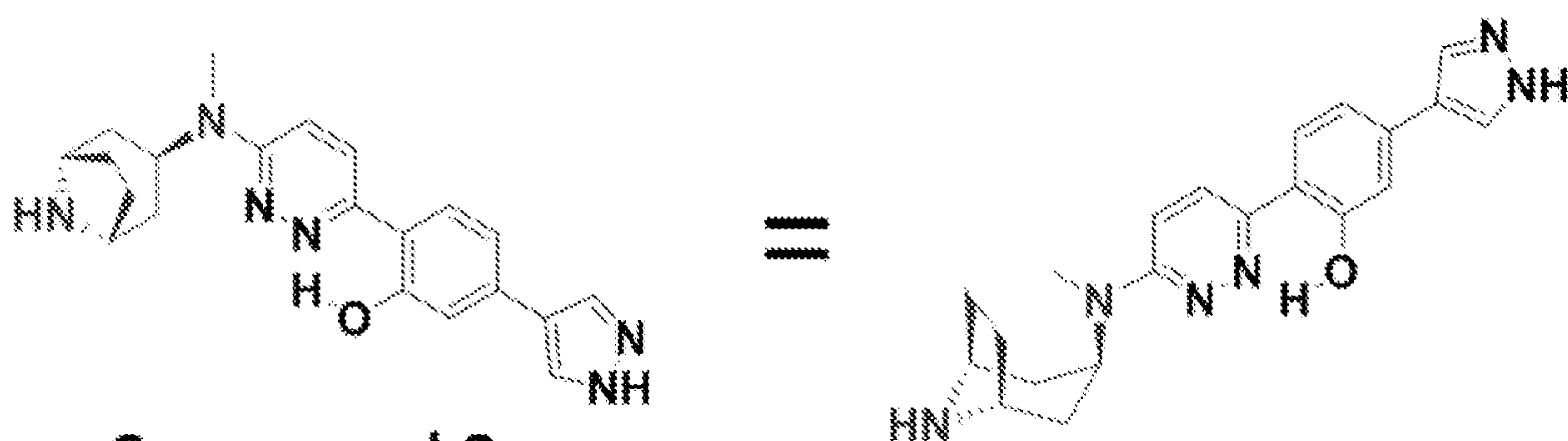
Compound 2
