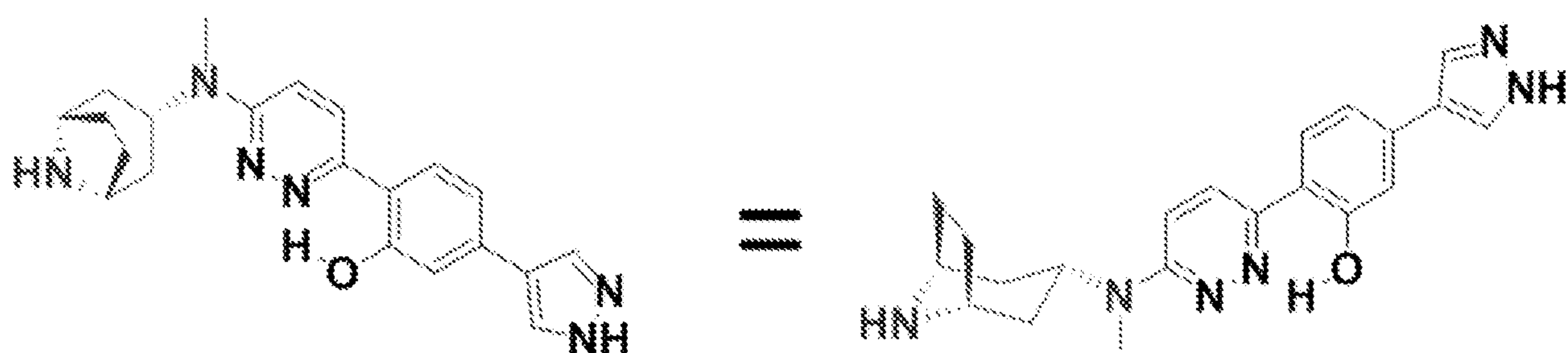
Compound 1
