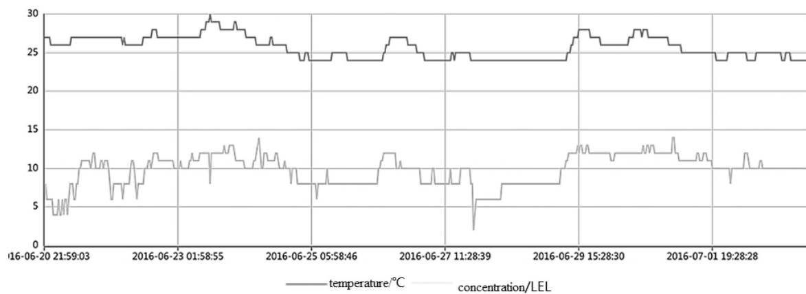
(b) example 2 of typical biogas leakage monitoring curve
