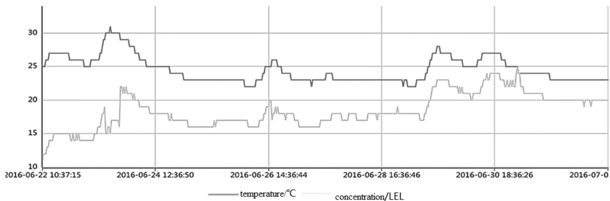
(a) example 1 of typical biogas leakage monitoring curve
