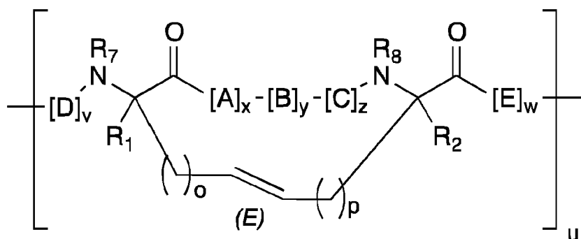
Formula (I),
