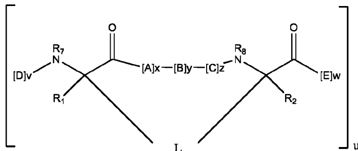
Formula I
