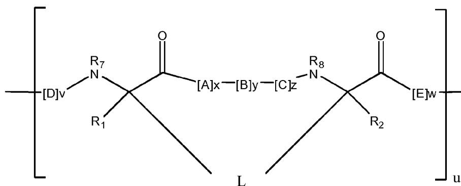
Formula (I)
