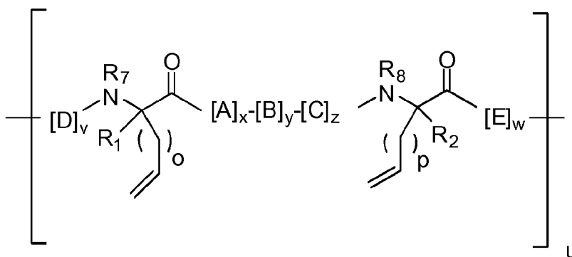
Formula (II),
