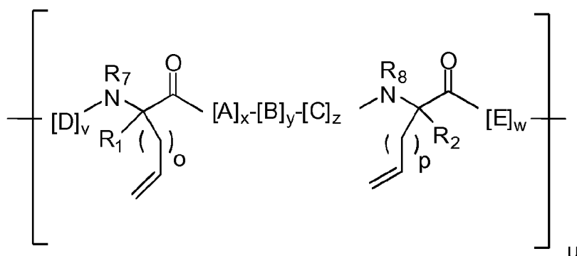
Formula (II),
