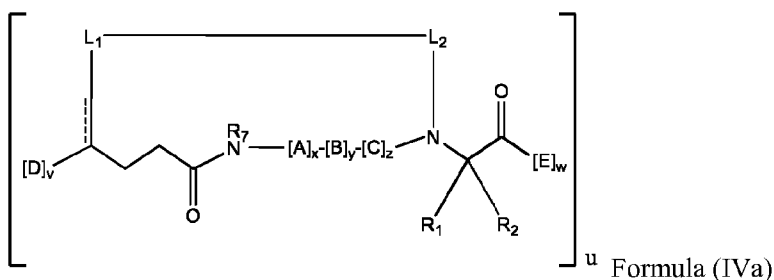
Formula (IV)
