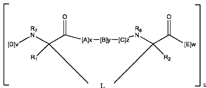
Formula I
