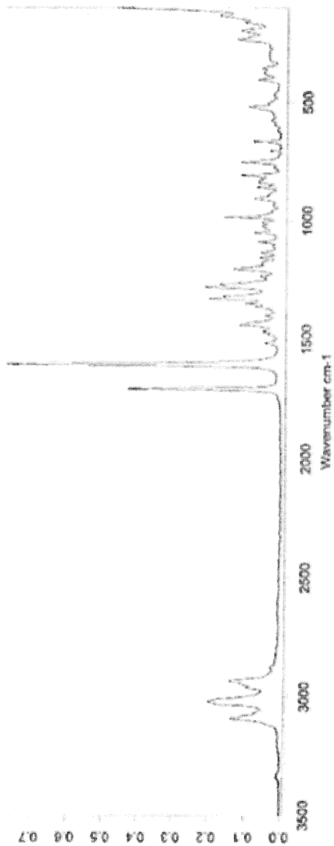
Fig. 2 - Raman spectrum of Compound (I), n=1 EtOH solvate
