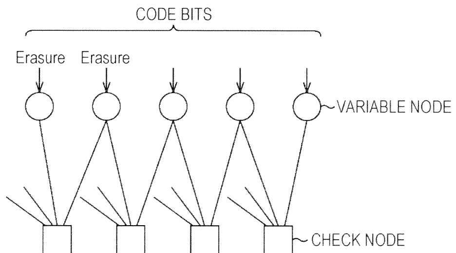
STEPWISE STRUCTURE PORTION OF TANNER GRAPH B
