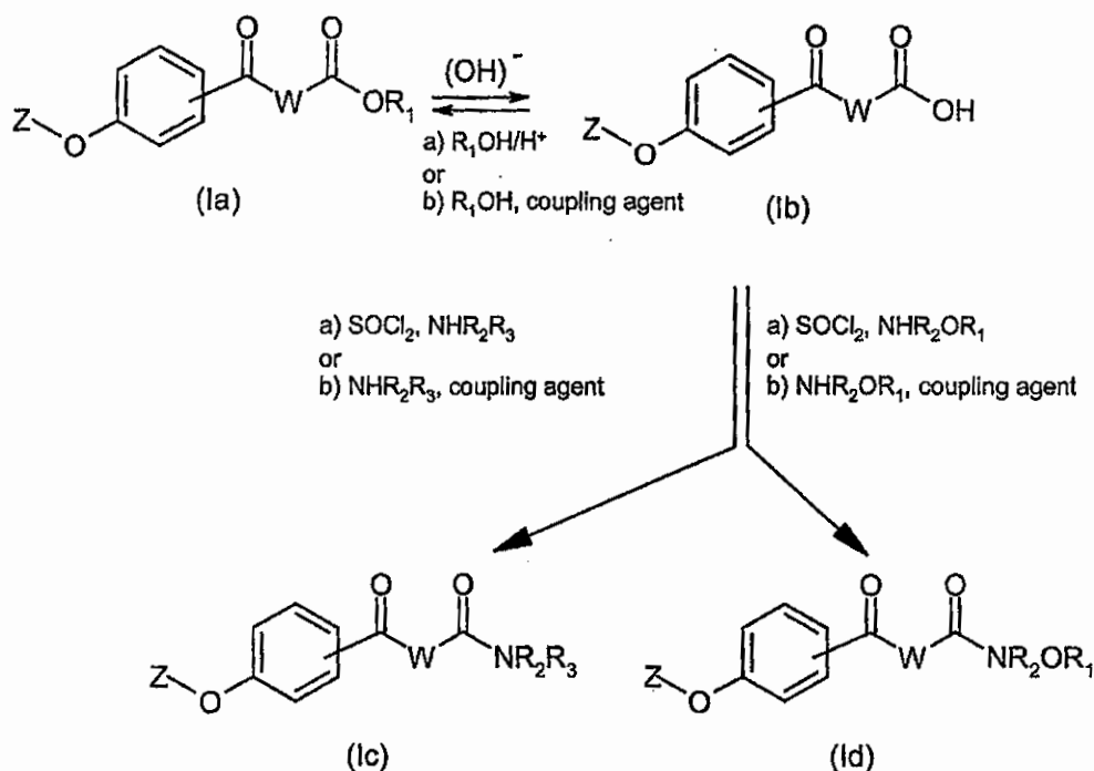
Scheme 6
