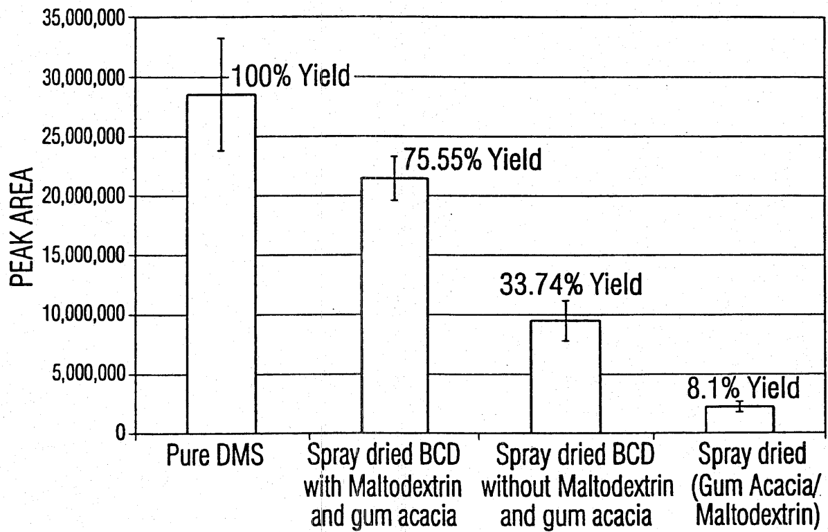
Peak Area of DMS as measured by GC Headspace on A J&W DB624 Column
