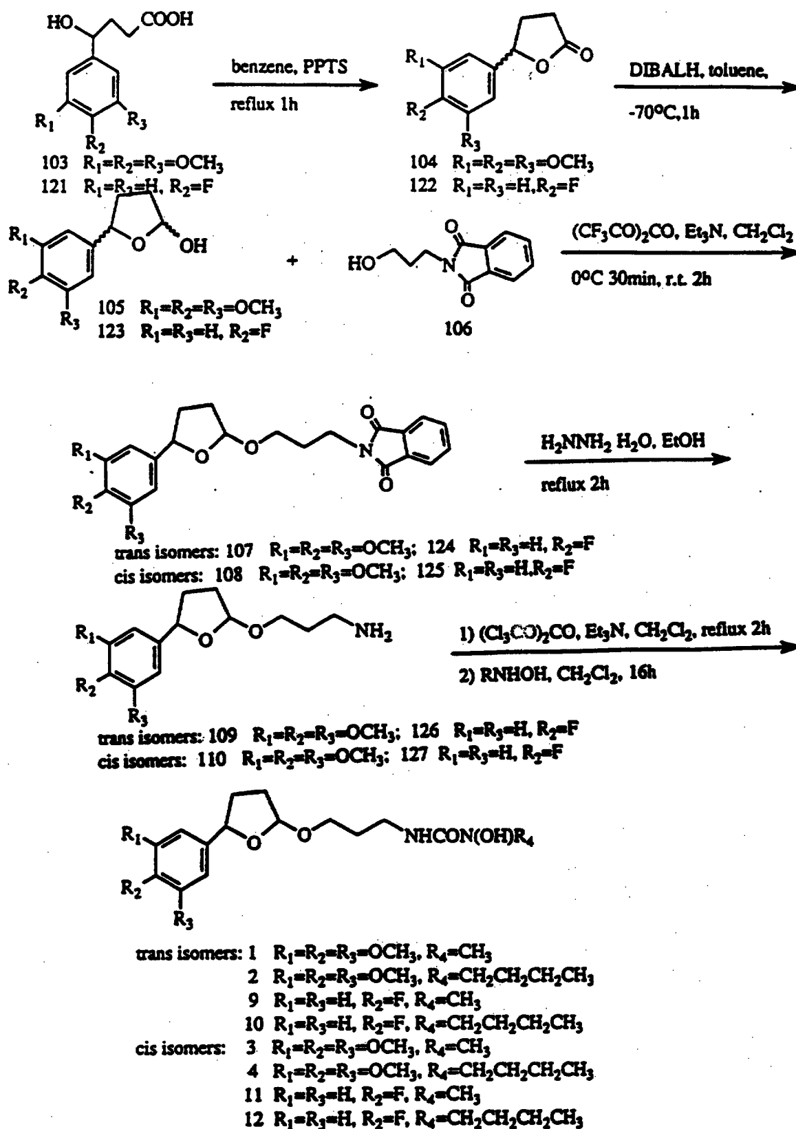
Scheme 5
