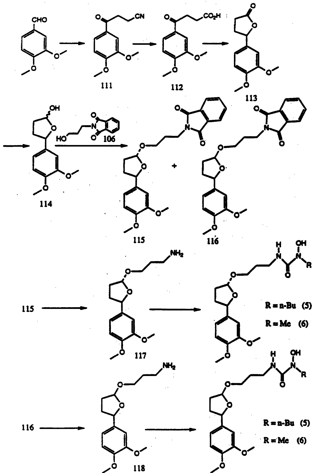
Scheme 7
