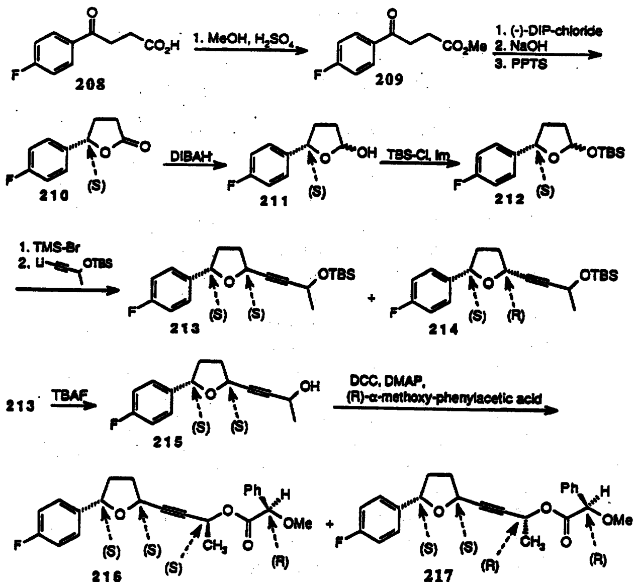
Scheme 9
