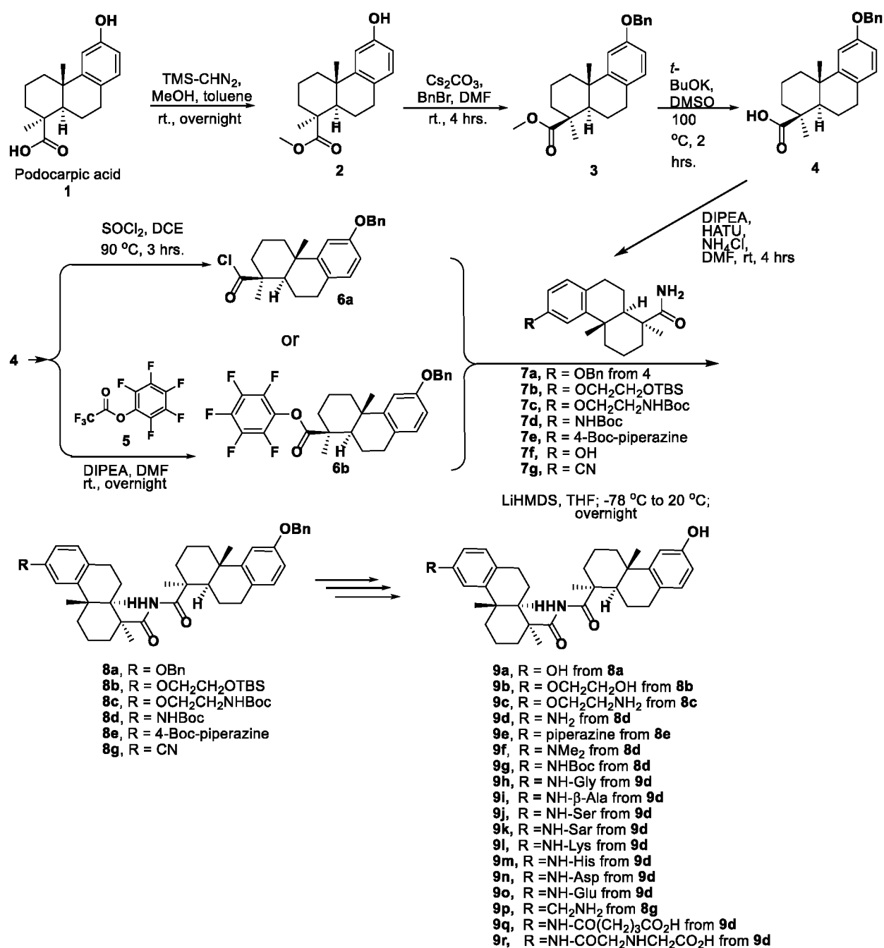
FIG. 1 Synthesis of 9a-9p
