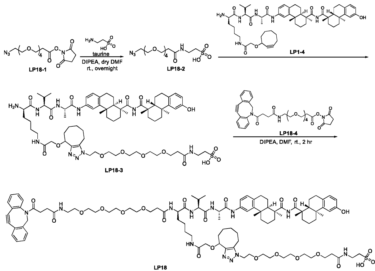
Figure 1f Synthesis of LP18
