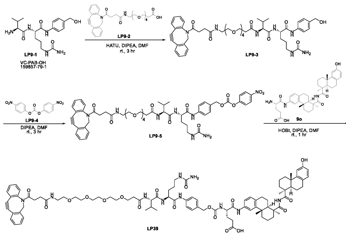
Figure 1i Synthesis of LP39
