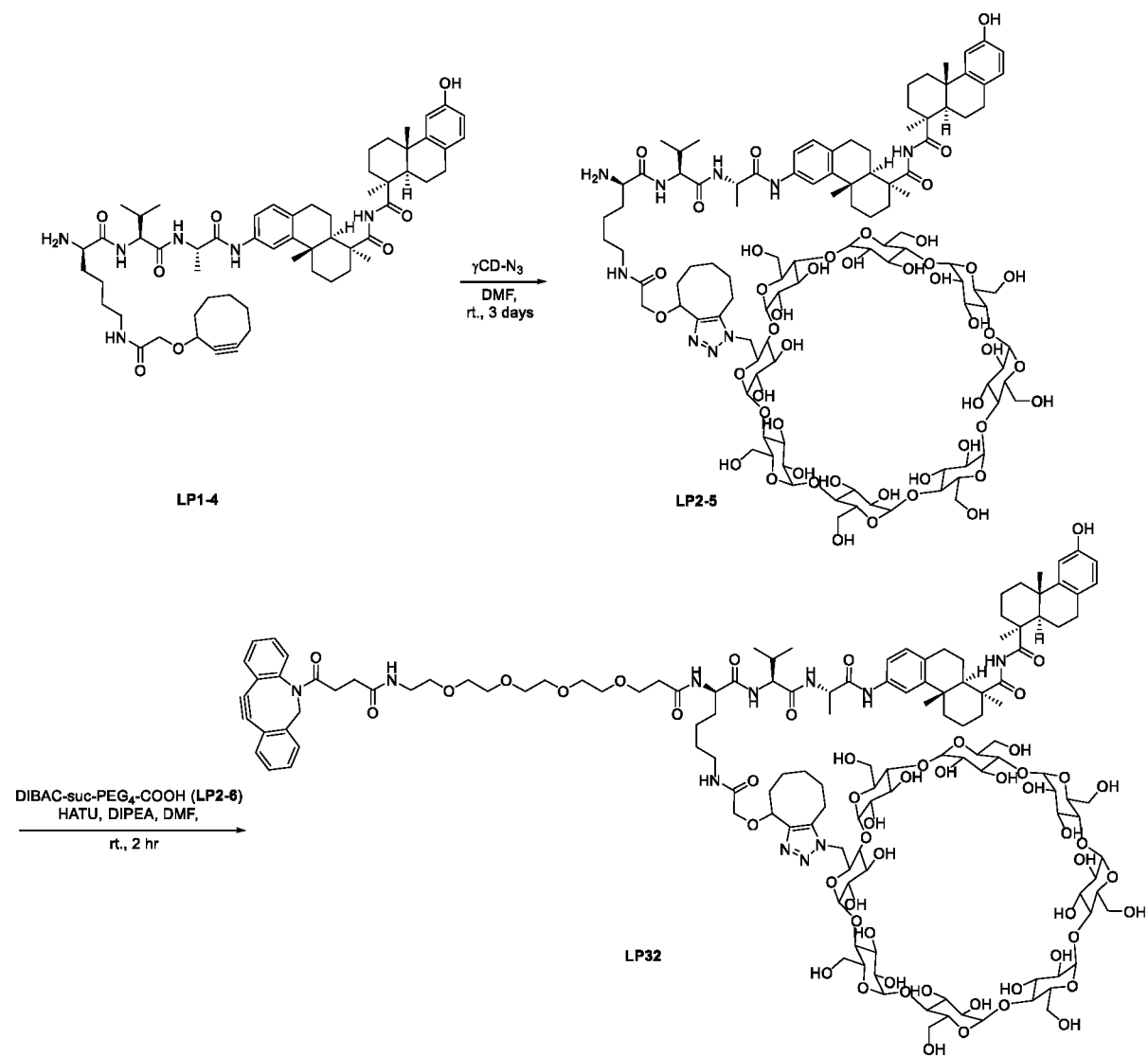
Figure 1c Synthesis of LP32
