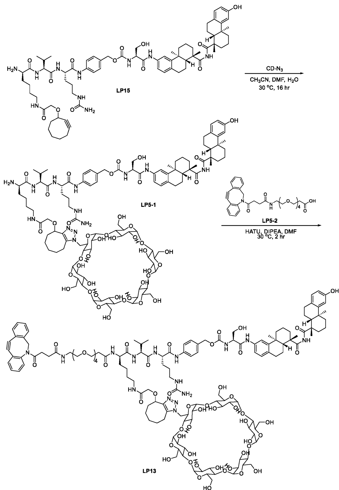
Figure 1d Synthesis of LP13
