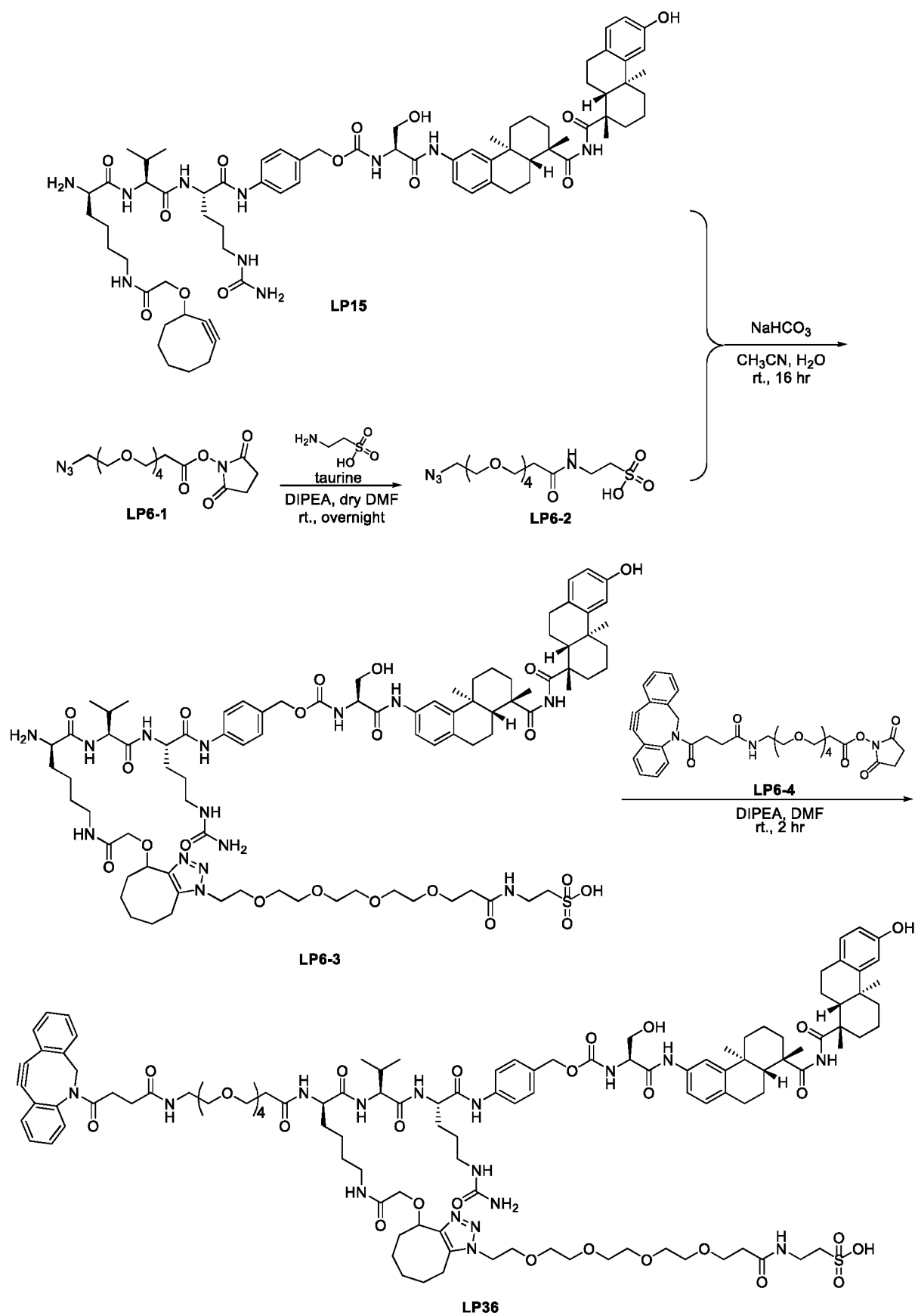
Figure 1e Synthesis of LP36
