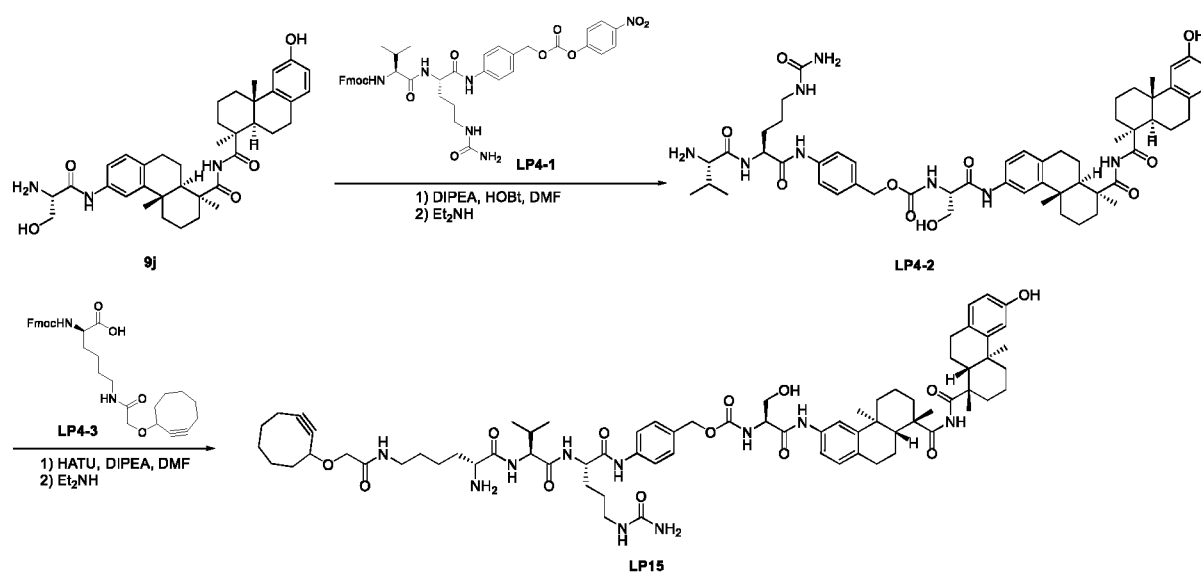
Figure 1g Synthesis of LP15
