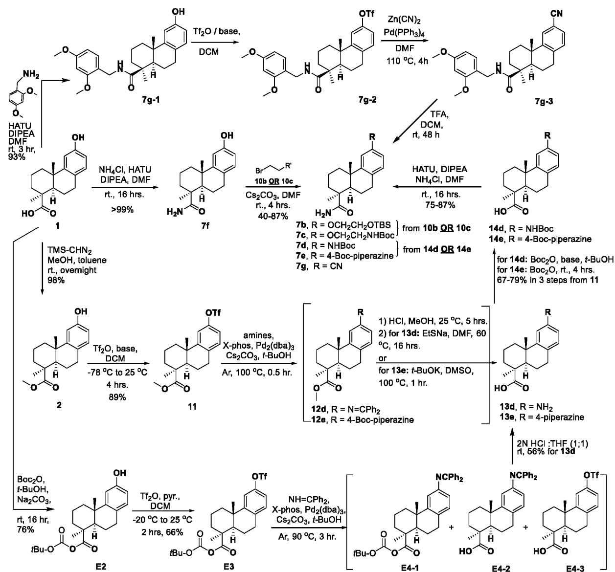
FIG. 2 Synthesis of Intermediates 7
