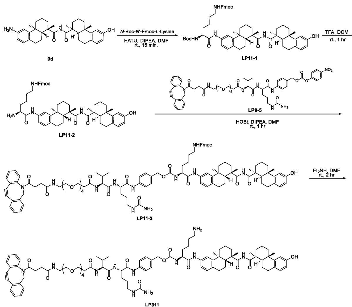
Figure 1h Synthesis of LP311
