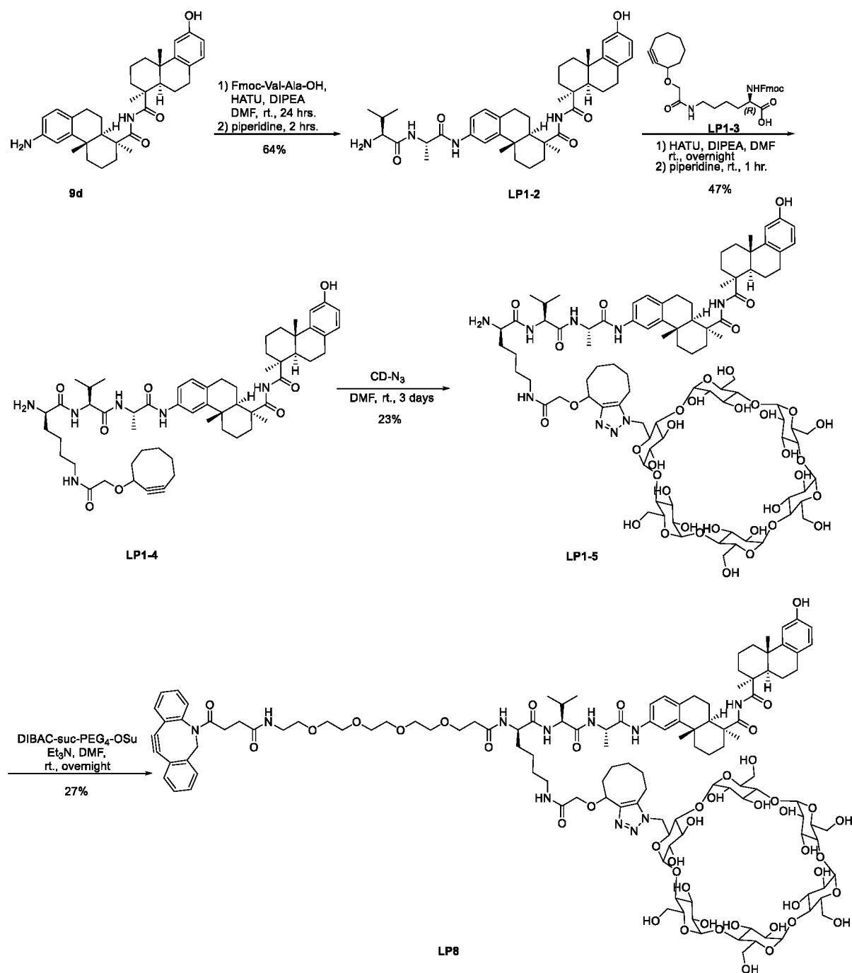
Figure 1b Synthesis of LP8
