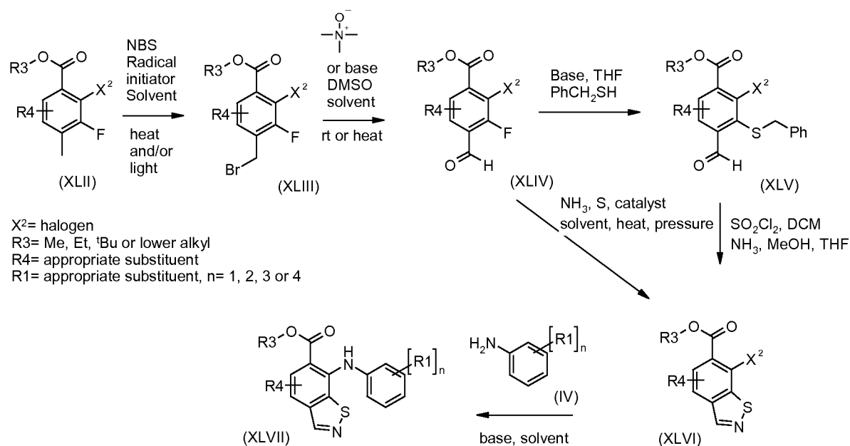
Scheme 10
