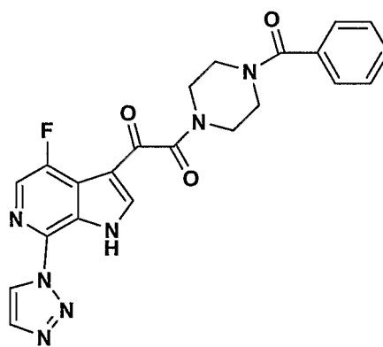
Compound IVb
