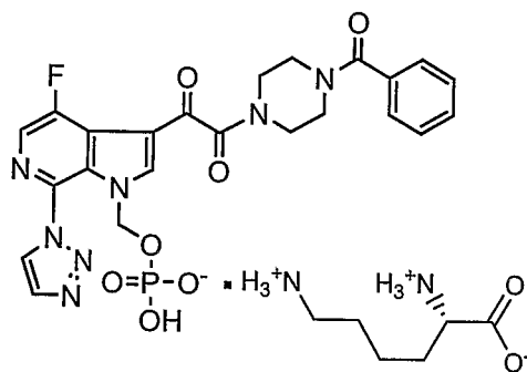
Ibb
