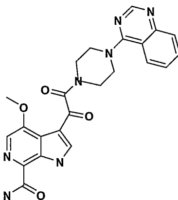
4-methoxy-3-(2-oxo-2-(4-(quinazolin-4-yl)piperazin-1-yl)acetyl)-1H-pyrrolo[2,3-c]pyridine-7-carboxamide
