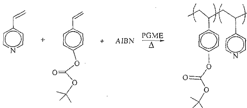
Scheme C
