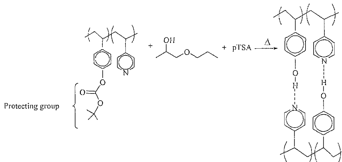
Scheme D
