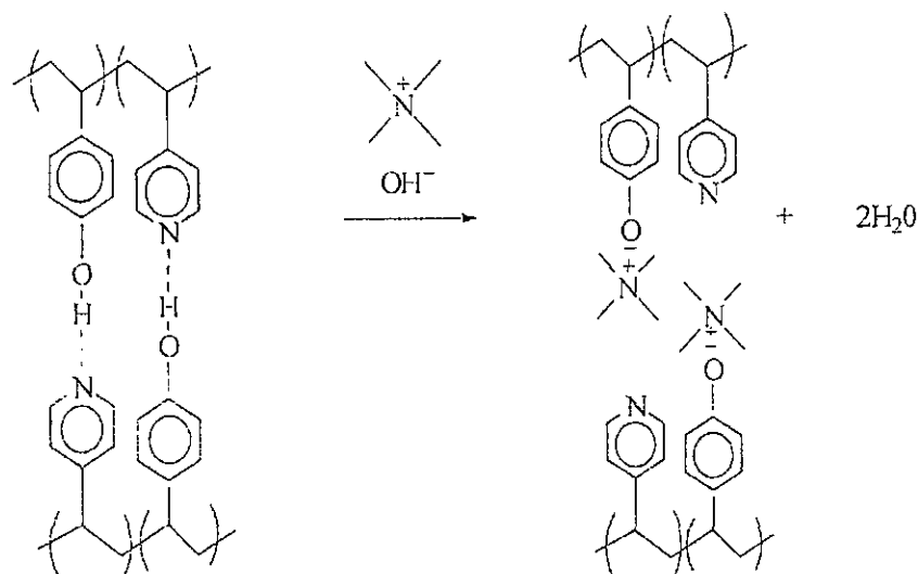
Scheme B
