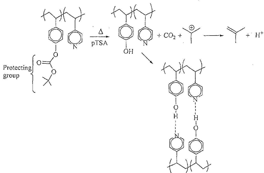
Scheme A
