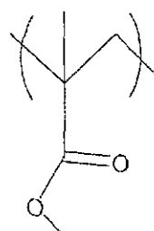
MMA monomer
