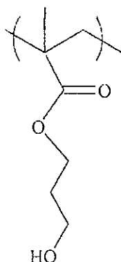
HPMA Monomer
